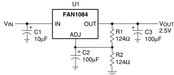
Figure 6. Application Circuit
