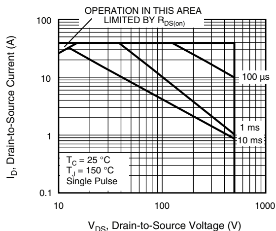
Fig. 1 - Maximum Safe Operating Area (TO-220AB, D2PAK)
