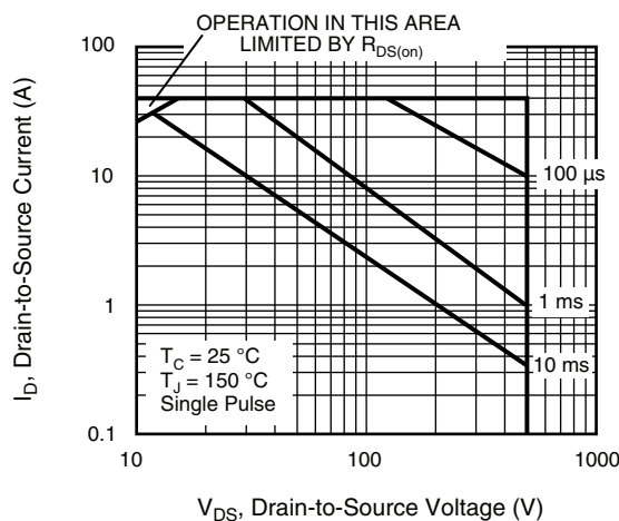
Fig. 2 - Maximum Safe Operating Area (TO-220 FULLPAK)
