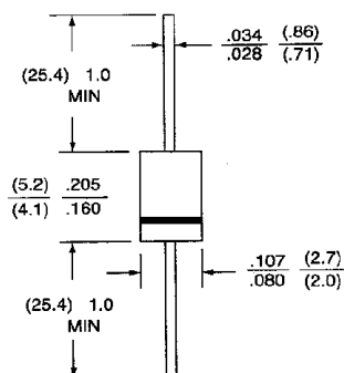
DO-41
