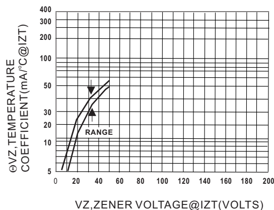
Fig.2-TEMPERATURE COEFFICIENT-RANGE
