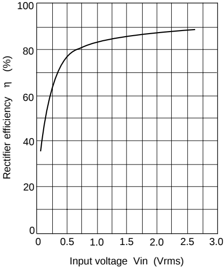
Fig.4 Rectifier efficiency Vs. Input voltage V_{in}
