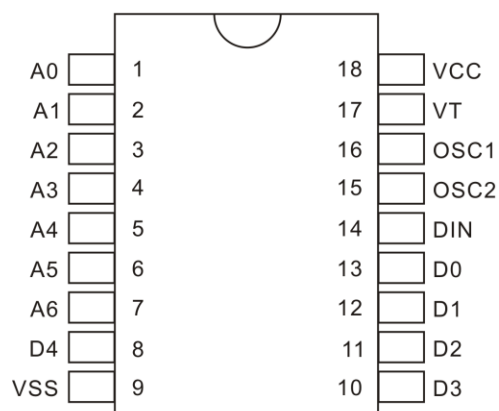
PT2272-M5/L5
