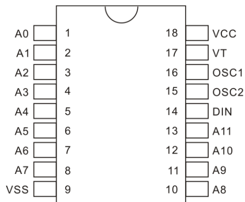
PT2272
