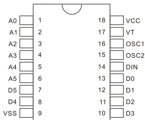
PT2272-M6
