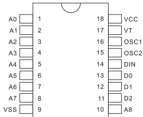
PT2272-M3/L3
