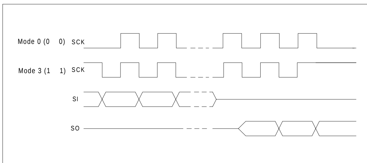
Figure 2. SPI Modes
