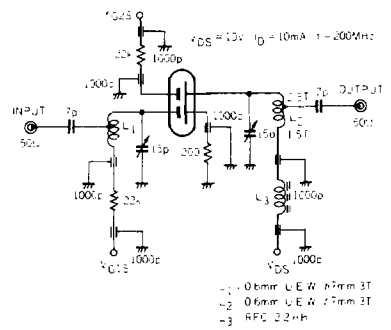
200MHz Power Gain & Noise Figure Test Circuit
