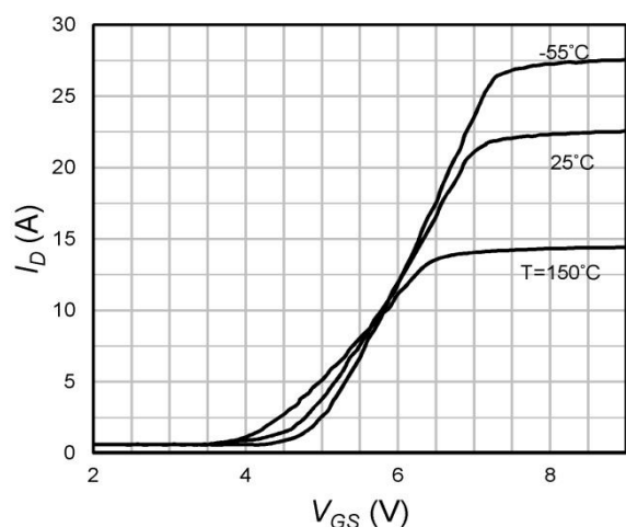
Fig.5 Transfer Characteristics
