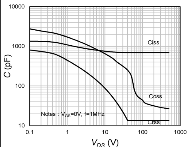
Fig.8 Capacitance Characteristics
