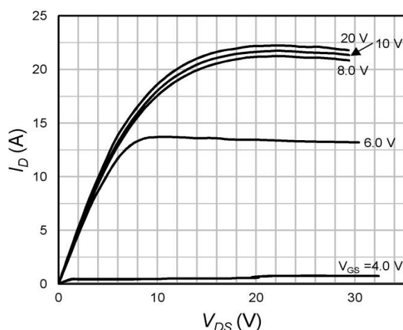
Fig.1 On-Region Characteristics.
