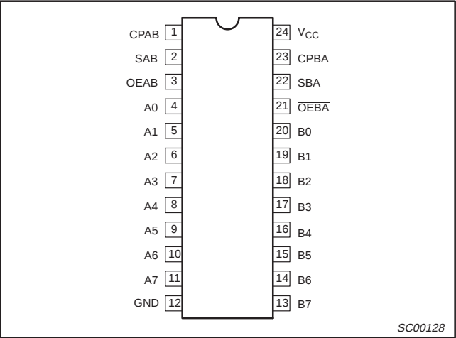
PIN CONFIGURATION – 74ALS652/652-1
