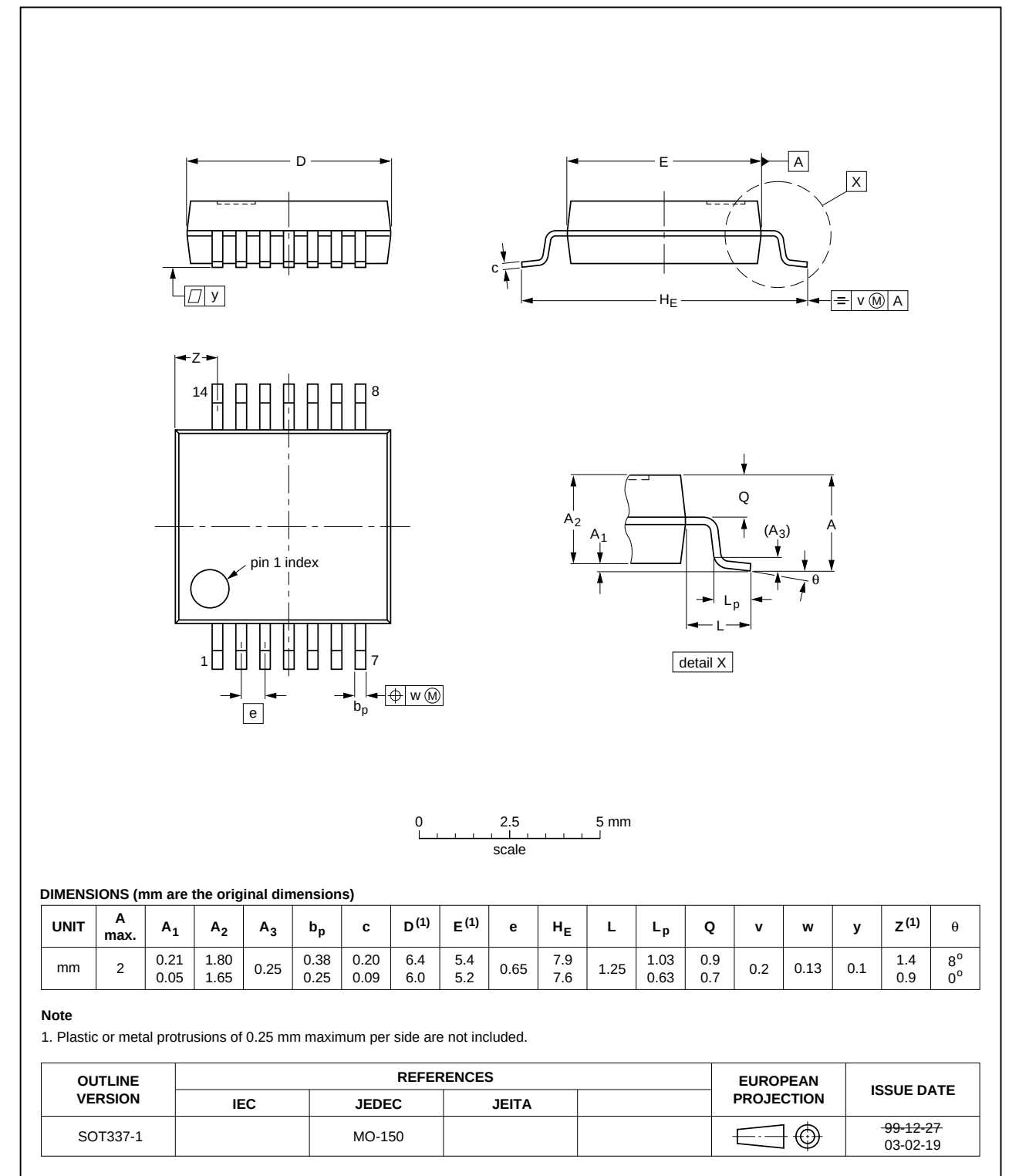
Fig 9. Package outline SOT337-1 (SSOP14)
