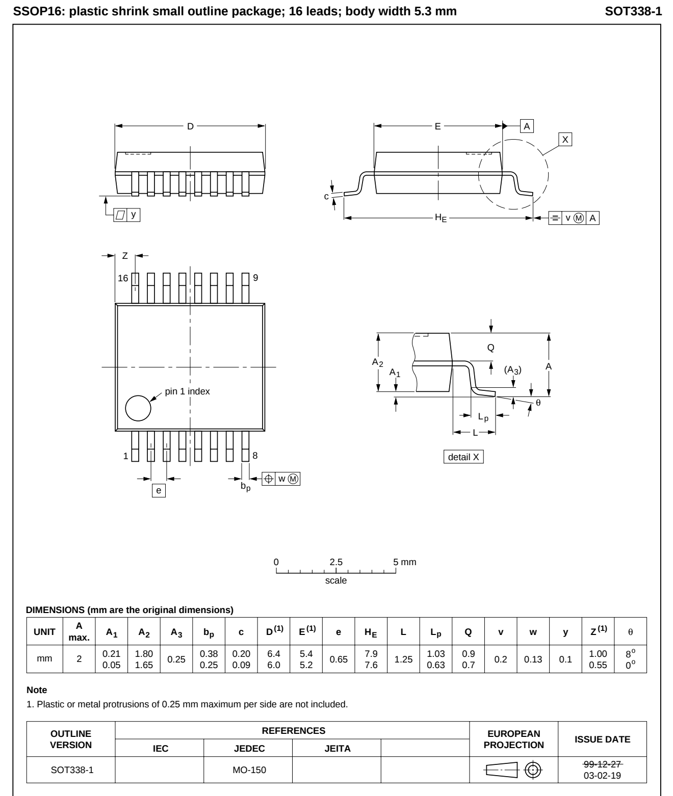
Fig 16. Package outline SOT338-1 (SSOP16)
