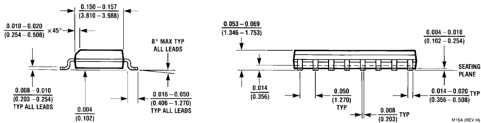
16-Lead Molded Package Small Outline (SO) Order Number DM74LS259M NS Package Number M16A
