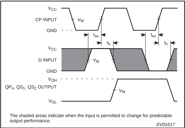
Figure 4. Data set-up and hold times for the data input (D).
