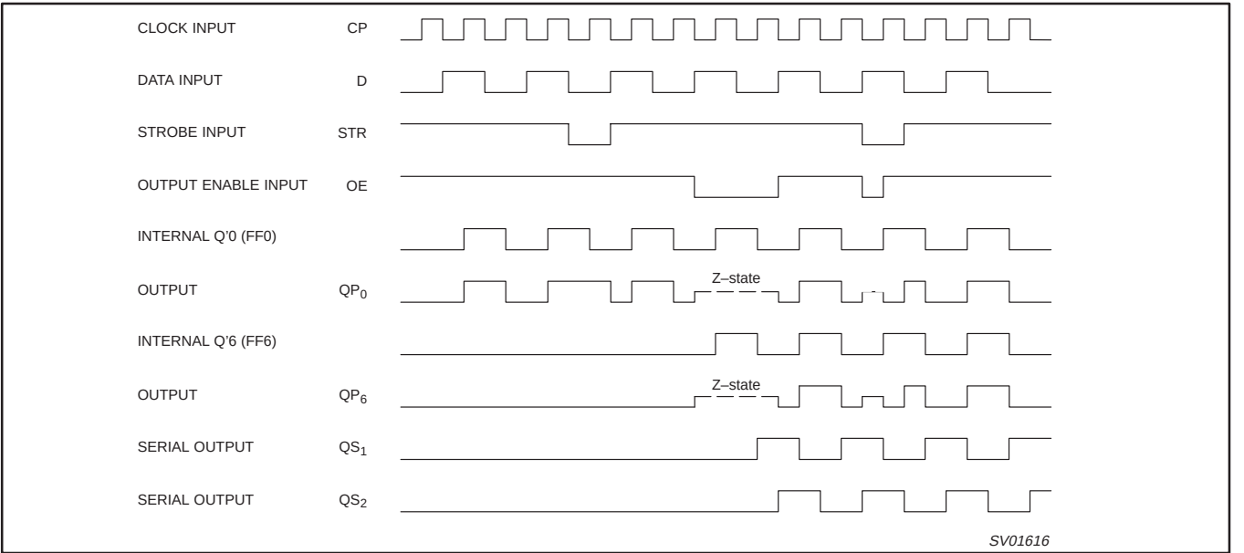
TIMING DIAGRAM
