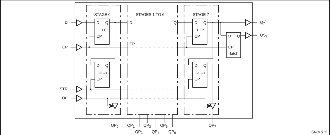
LOGIC DIAGRAM
