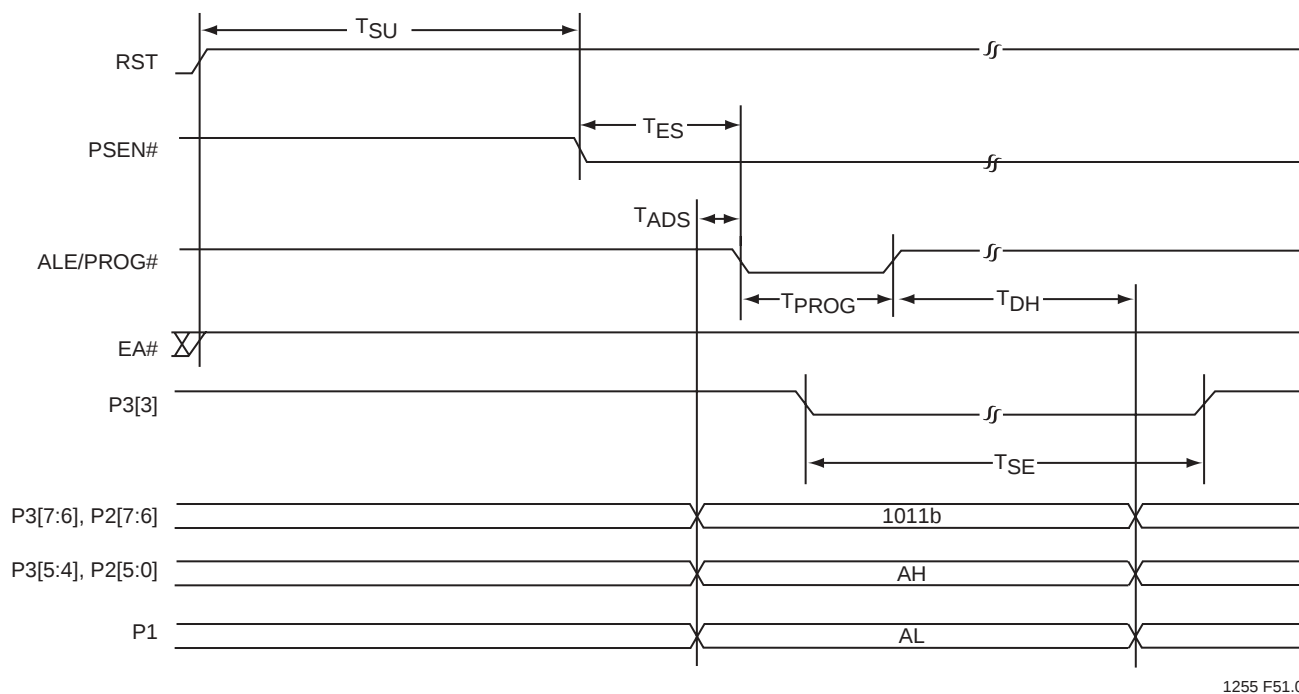
FIGURE 14-19: SECTOR-ERASE
