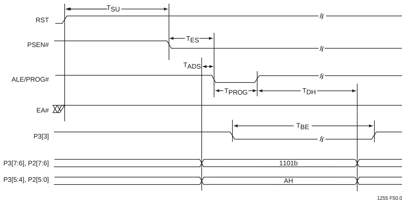
FIGURE 14-18: BLOCK-ERASE FOR SST89E5xRD2/SST89V5xRD2
