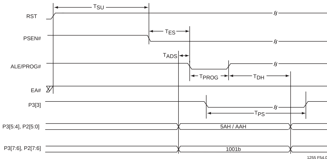
FIGURE 14-22: Prog-SC0 / Prog-SC1
