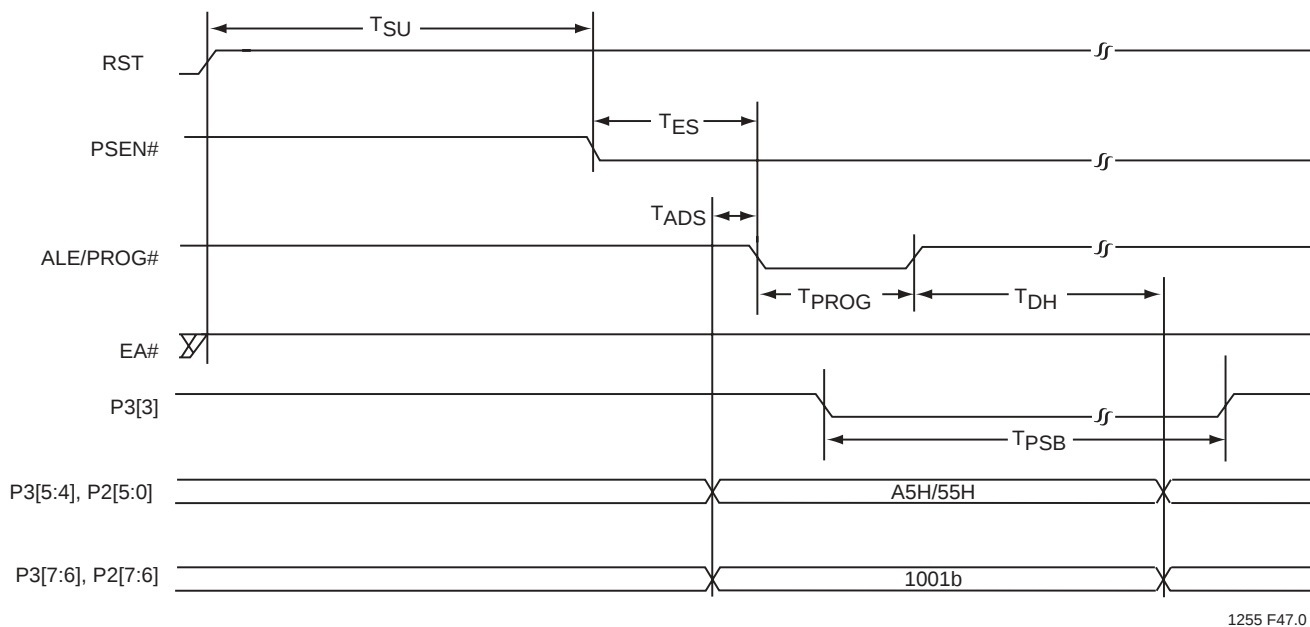
FIGURE 14-15: SELECT-BLOCK1 / SELECT-BLOCK0 (FOR SST89E516RD2/SST89V516RD2 ONLY)
