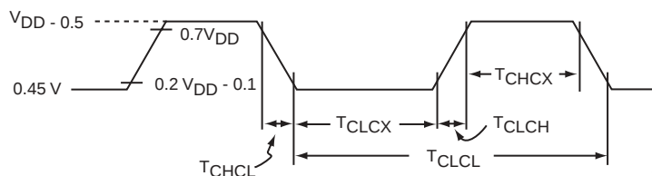
FIGURE 14-6: EXTERNAL CLOCK DRIVE WAVEFORM
