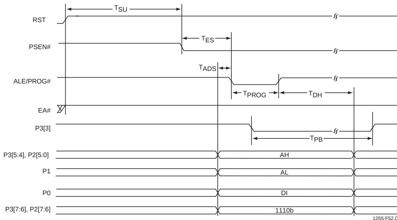
FIGURE 14-20: BYTE-PROGRAM
