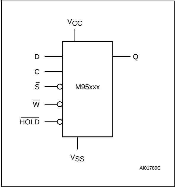
Figure 2. Logic Diagram
