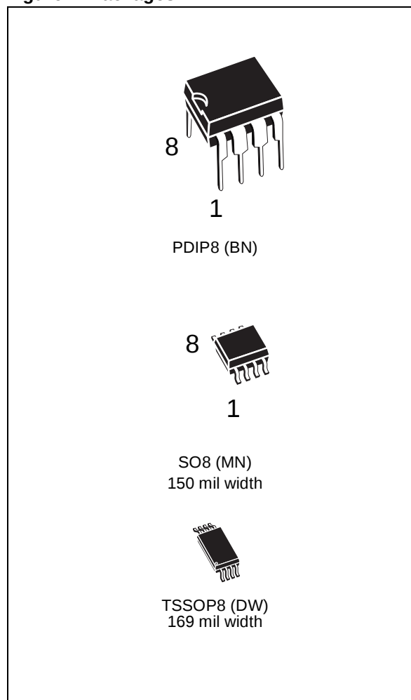
Figure 1. Packages
