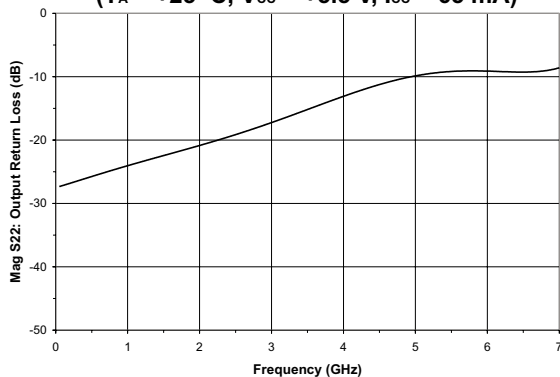
Figure 7: Output Return Loss vs. Frequency De-embedded 50 \Omega S-parameter (T A = +25 °C, V CC = +5.5 V, I CC = 65 mA)
