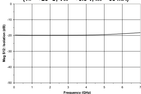
Figure 5: Isolation vs. Frequency De-embedded 50 \Omega S-parameter (T A = +25 °C, V CC = +5.5 V, I CC = 65 mA)
