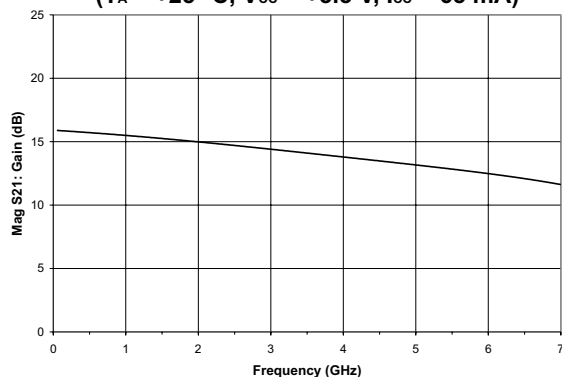
Figure 4: Gain vs. Frequency De-embedded 50 \Omega S-parameter (T A = +25 °C, V CC = +5.5 V, I CC = 65 mA)
