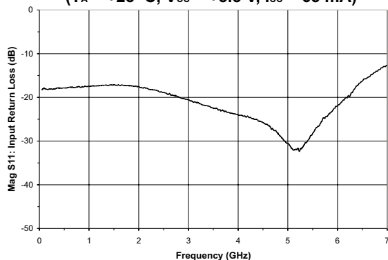
Figure 6: Input Return Loss vs. Frequency De-embedded 50 \Omega S-parameter (T A = +25 °C, V CC = +5.5 V, I CC = 65 mA)
