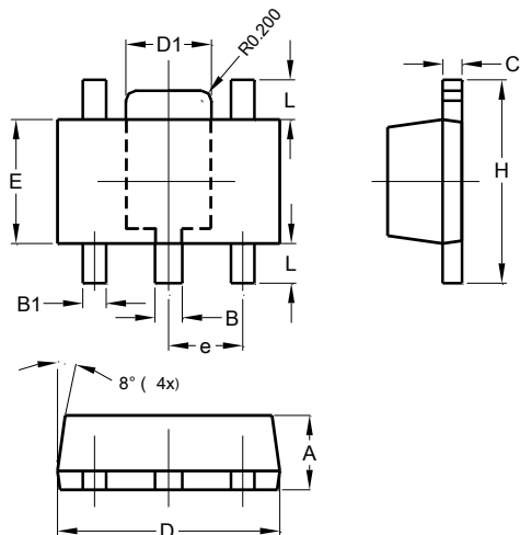
SOT89-5
