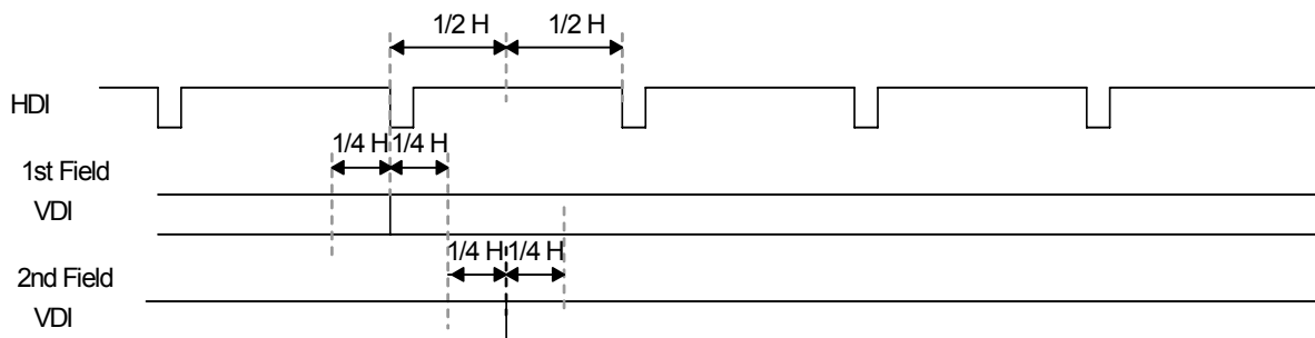
Fig. 157 HD/VD timing
