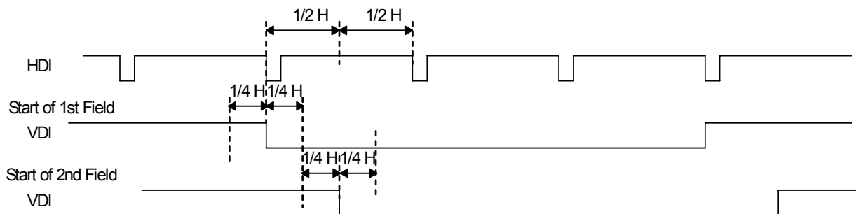
Fig. 83 Recognition of Field
