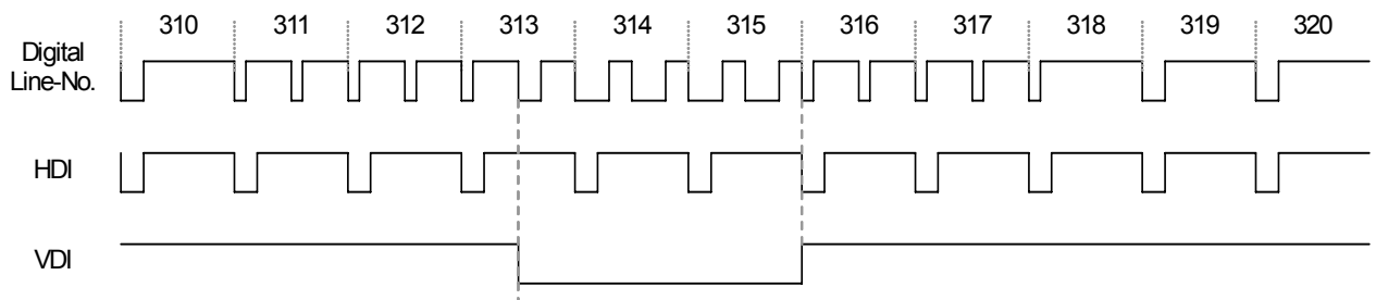
Fig. 161 2nd Field
