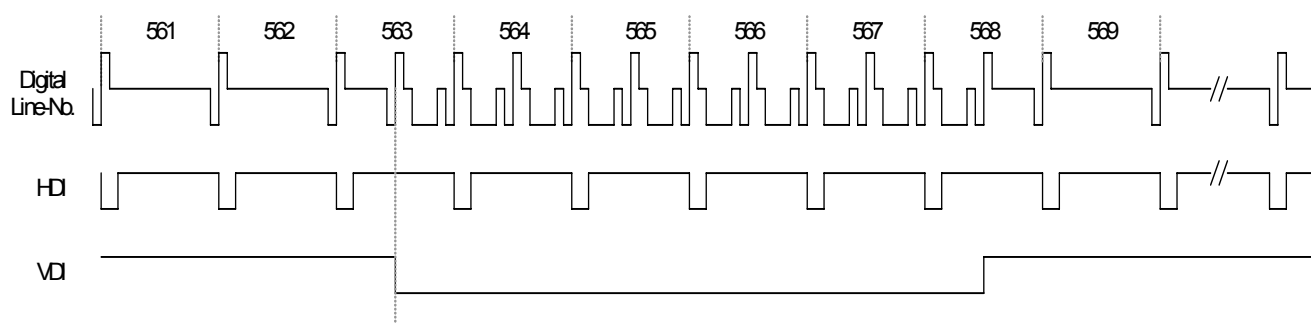
Fig. 97 1080i Relation between HSYNC and VSYNC (2)
