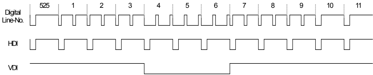
Fig. 158 1st Field
