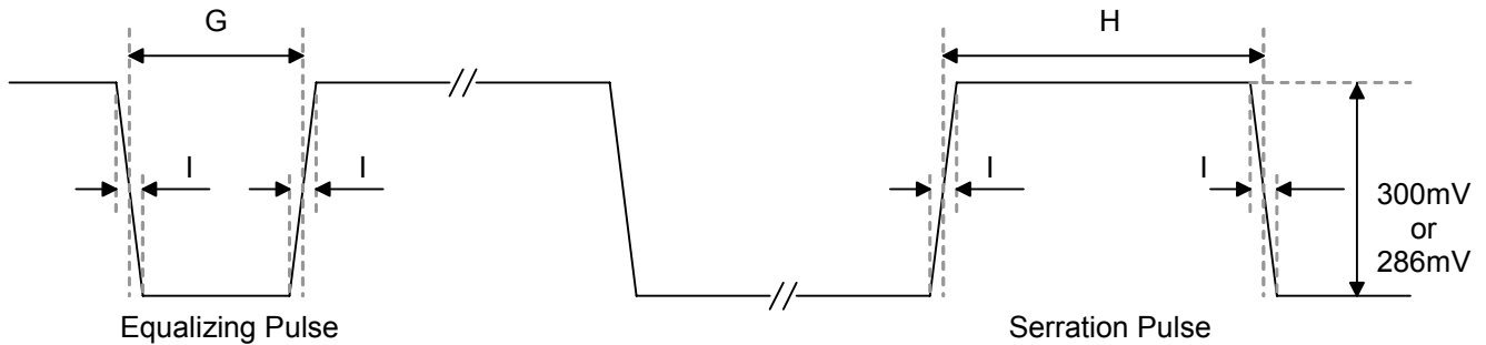
Fig. 123 Equalizing Pulse と Serration Pulse
