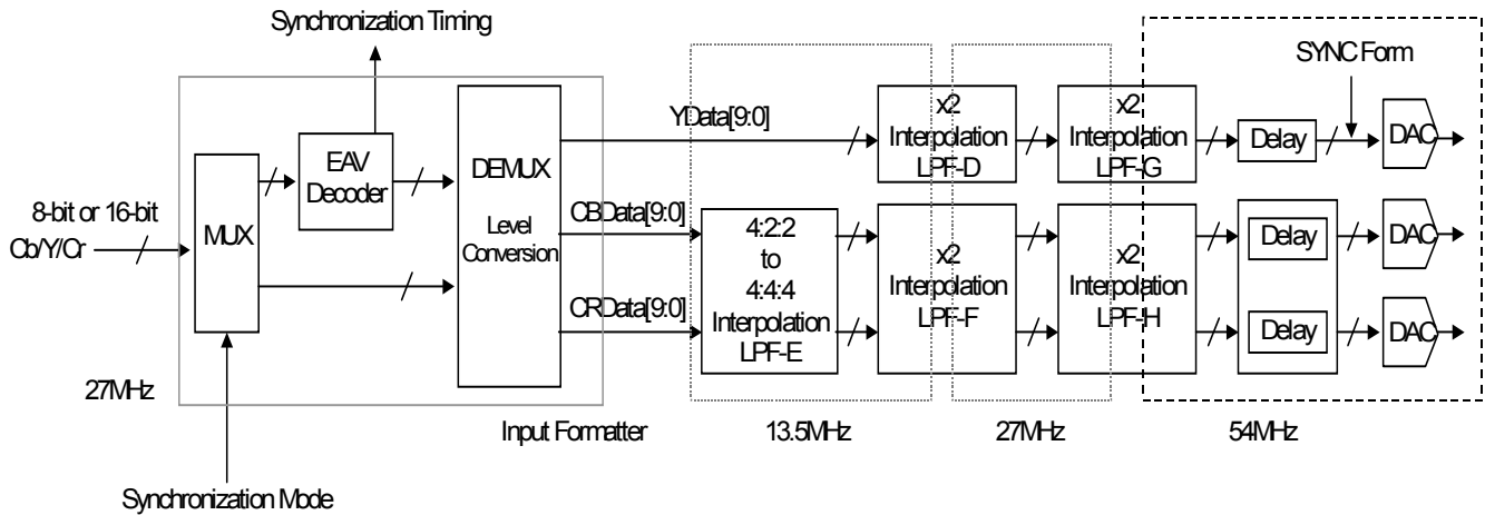
Fig. 37 525i/625i mode Block Diagram
