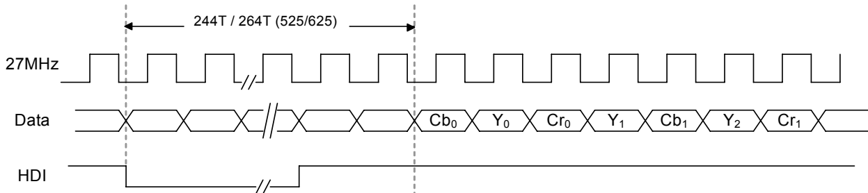
Fig. 156 Relation between HSYNC and Data
