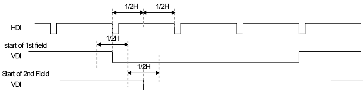
Fig. 105 Field Recognition
