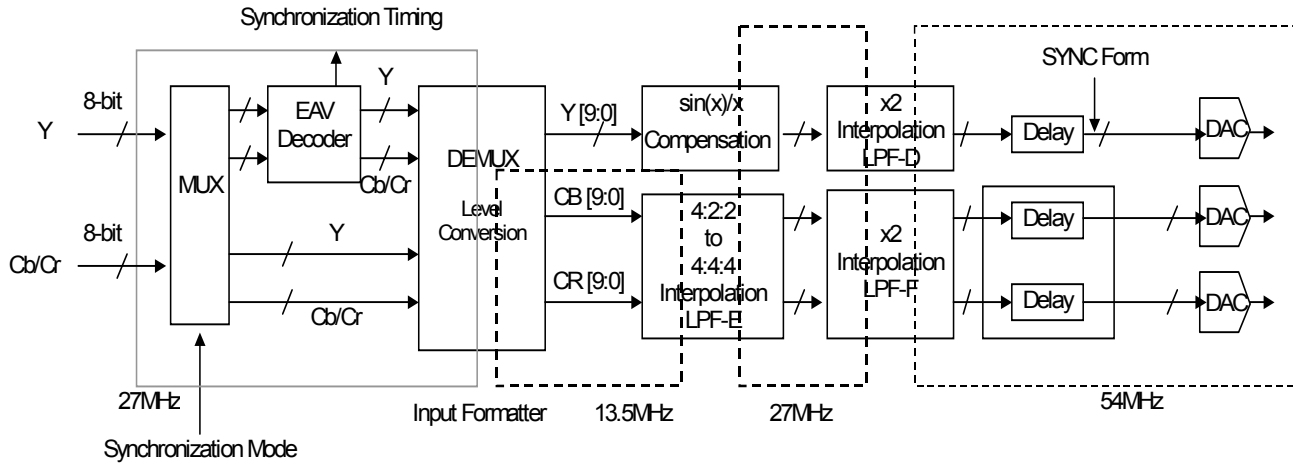
Fig. 41 525P/625P mode Block Diagram
