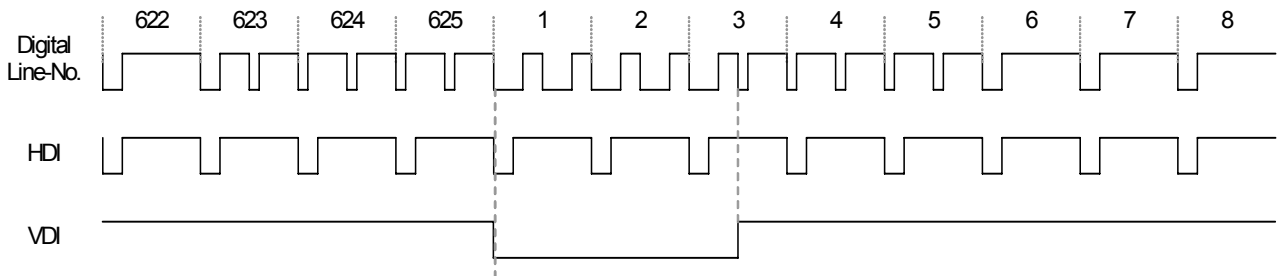
Fig. 160 1st Field
