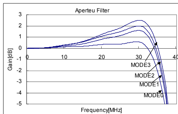
Fig. 46 Aperture Filter
