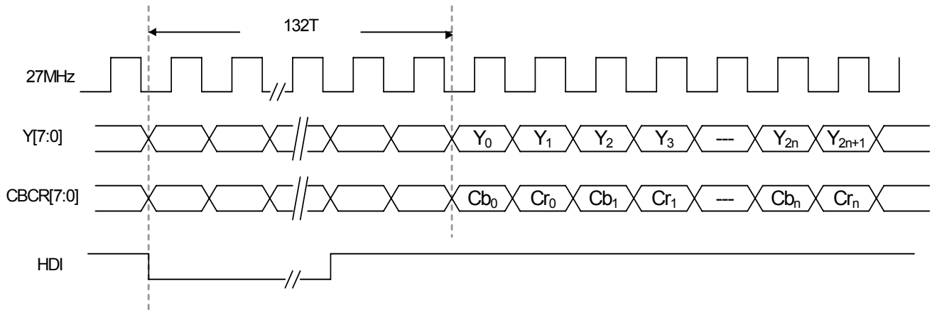
Fig. 92 625p HSYNC and data (8-bit x 2ch)
