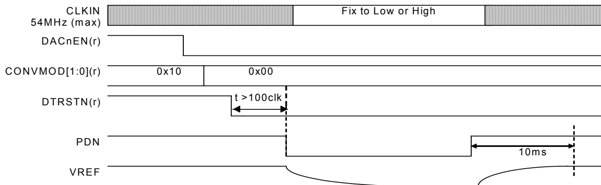
Fig. 18 Power-Down and power-down release Sequence from Component Video Encoder mode
