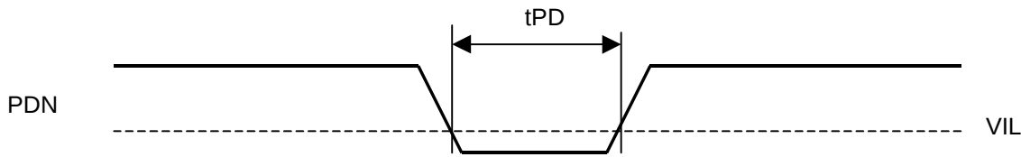
Power-down Timing
