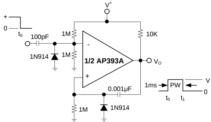
One-Shot Multivibrator
