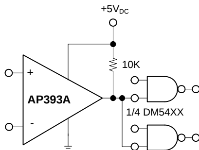
Driving TTL
