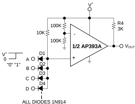
AND Gate
