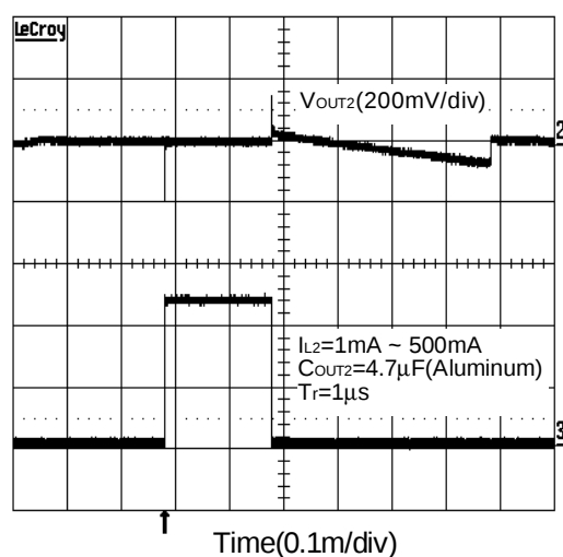
Load-Transient Response
