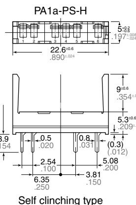
Self clinching type
