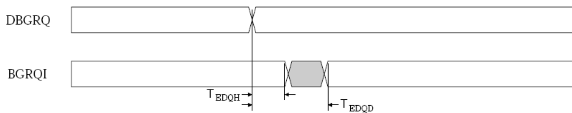
Figure 8-19 ARM9TDMI EDBGQRQ to DBGRQI relationship
