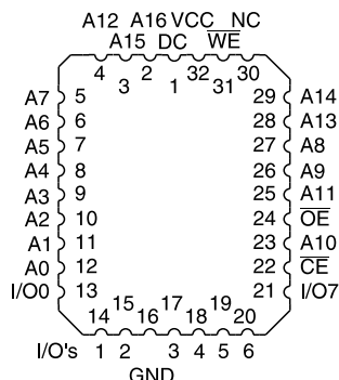
PLCC Top View
