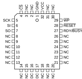
PLCC
