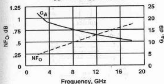
Noise Figure and Associated Gain vs. Frequency (ATF-35076) V_{DS} = 1.5\text{ V} , I_{DS} = 20\text{ mA}
