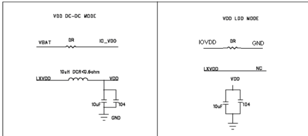
Figure 16-2-1 Li-Ion Supply Peripheral Connection
