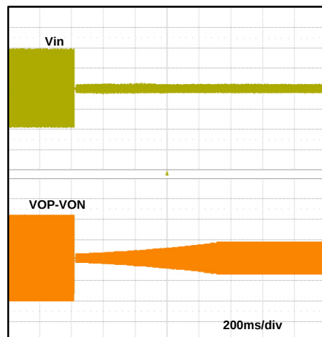
SINGLE-LEVEL-AGC 功能释放时序
