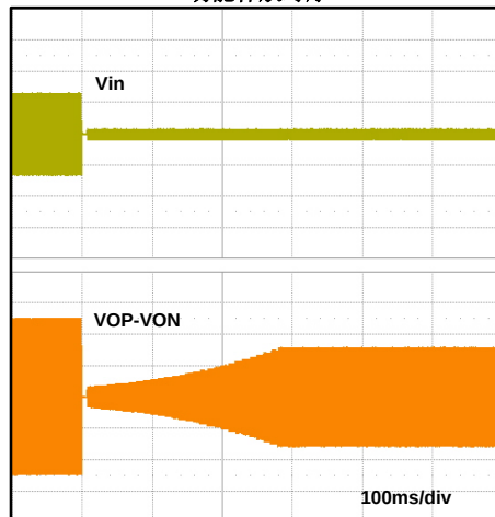
MULTI-LEVEL-AGC 功能释放时序
