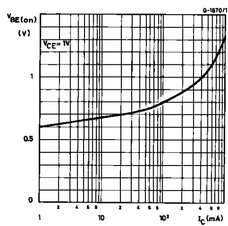
Base-emitter Voltage.
