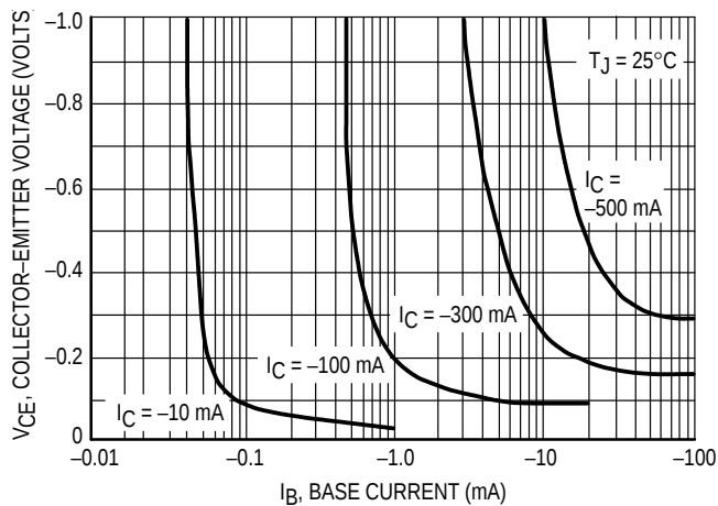
Figure 4. Saturation Region
