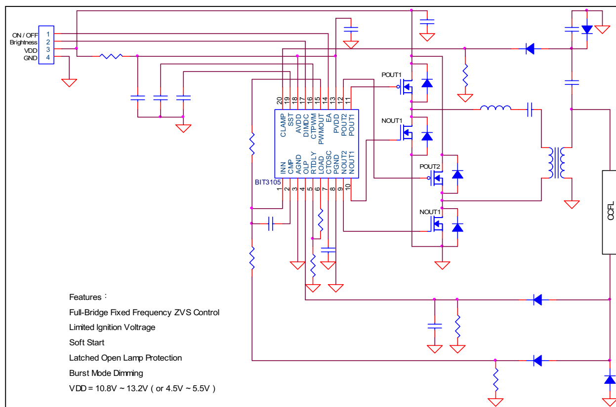
A Typical application of BIT3105
