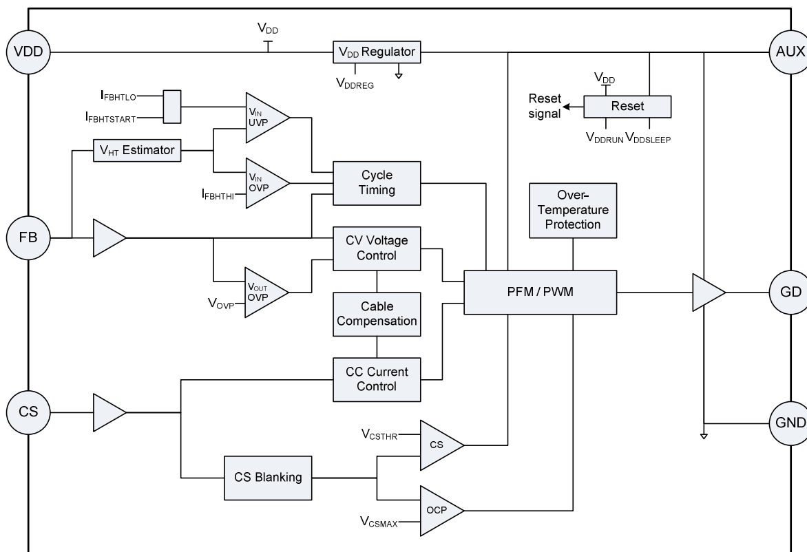
Figure 2: C2183 Block Diagram
