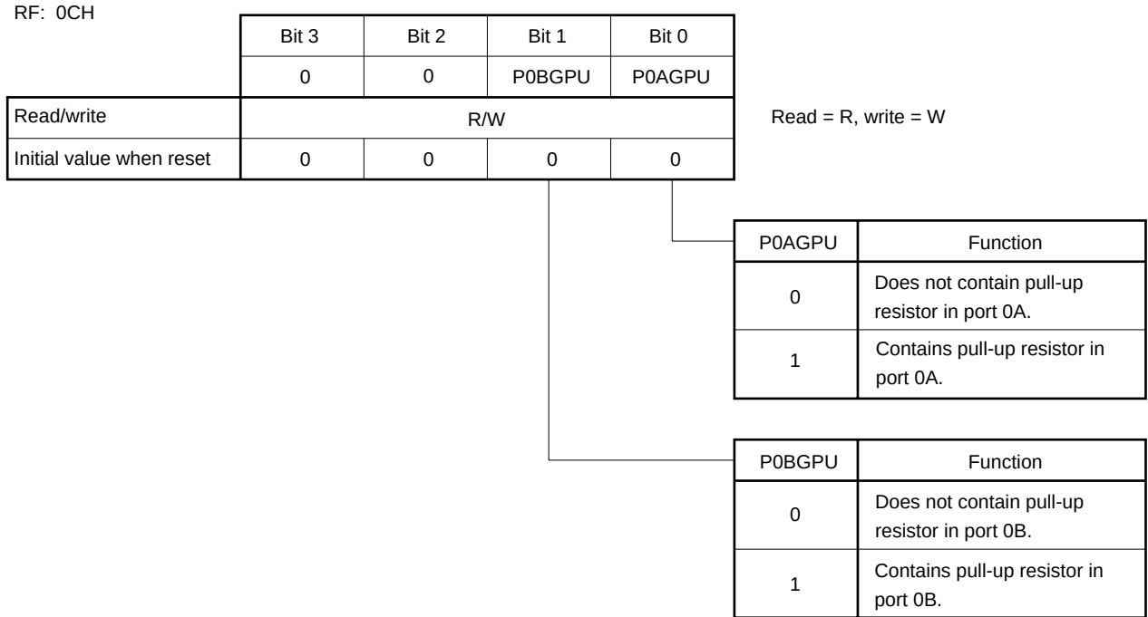
Figure 12-3. Specifying Pull-Up Resistor Incorporation Using Software
