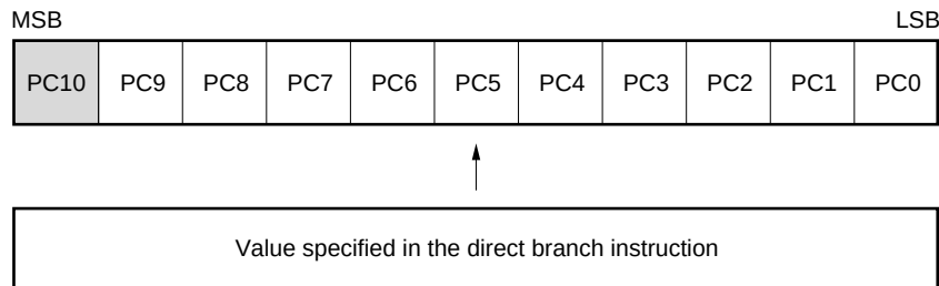
Figure 3-4. Value in the Program Counter during Execution of a BR addr Instruction
