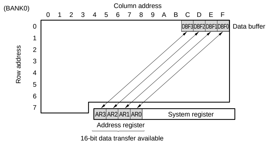
Figure 7-4. Address Register Used as a Peripheral Circuit
