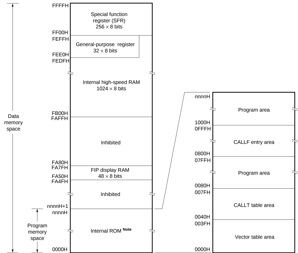
Fig. 4-1 Memory Map
