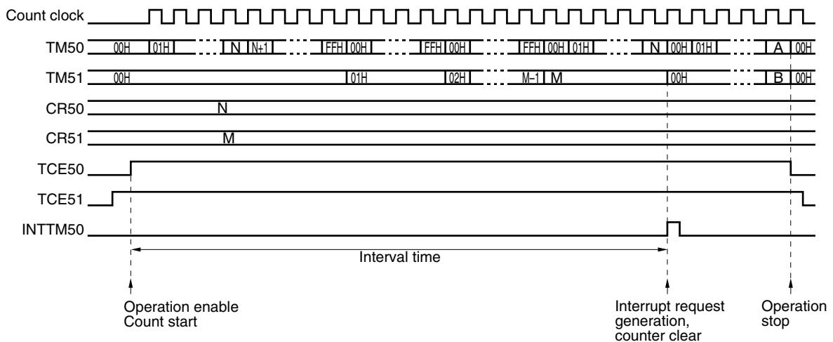
★ Figure 9-15. 16-Bit Resolution Cascade Connection Mode
