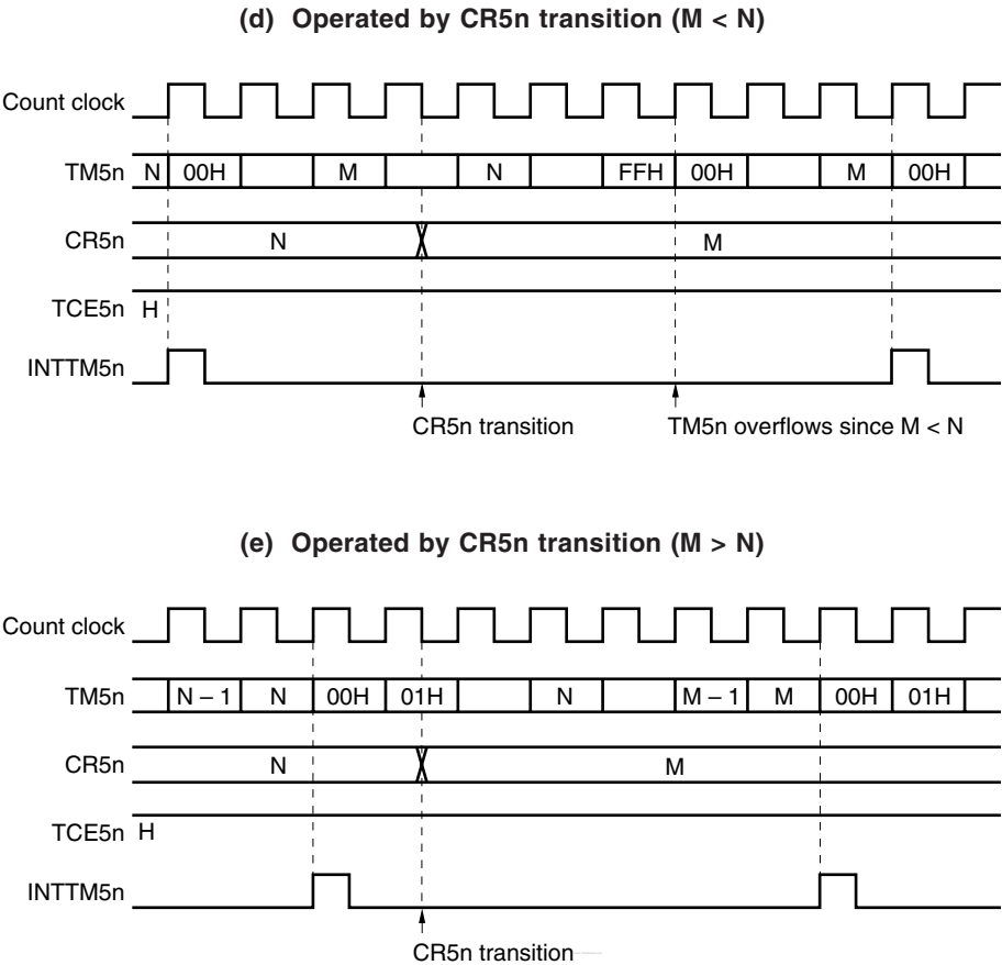
Figure 9-10. Interval Timer Operation Timing (3/3)
