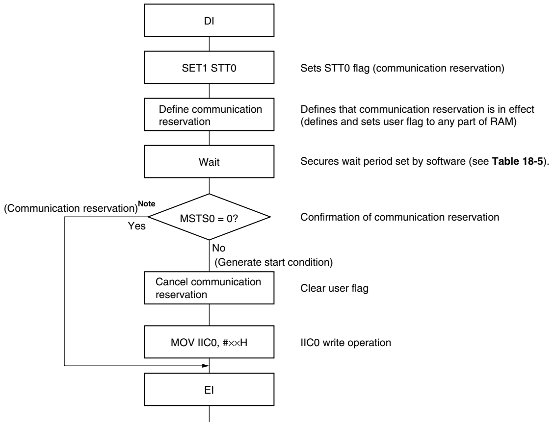
Figure 18-20. Communication Reservation Protocol
