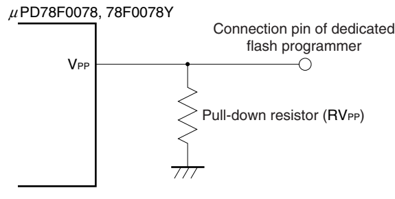
Figure 23-6. V PP Pin Connection Example
