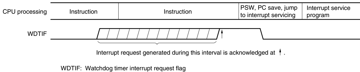
Figure 19-8. Non-Maskable Interrupt Request Acknowledgment Timing
