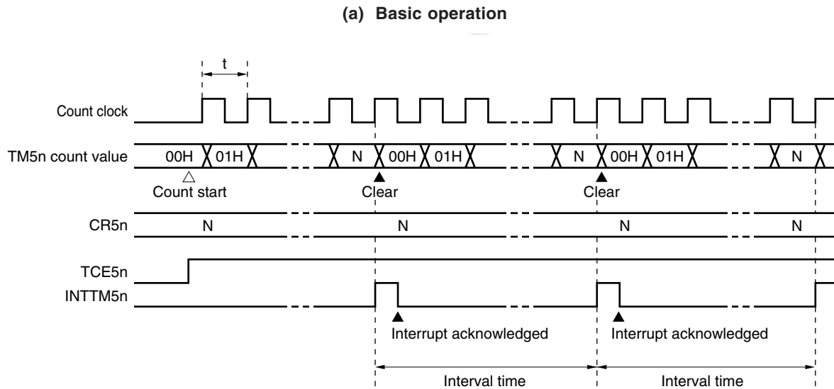
Figure 9-10. Interval Timer Operation Timing (1/3)
