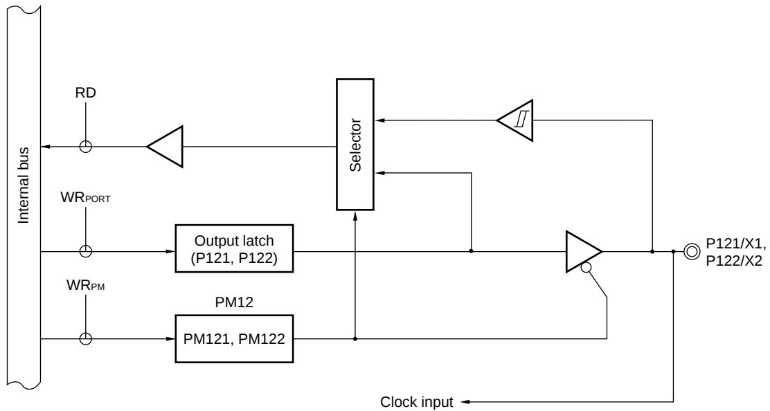
Figure 4-10. Block Diagram of P121 and P122
