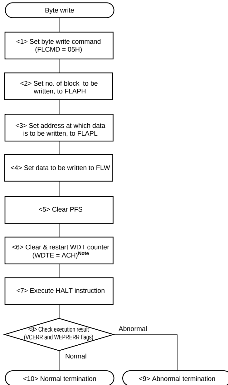
Figure 18-24. Example of Byte Write Operation in Self Programming Mode
