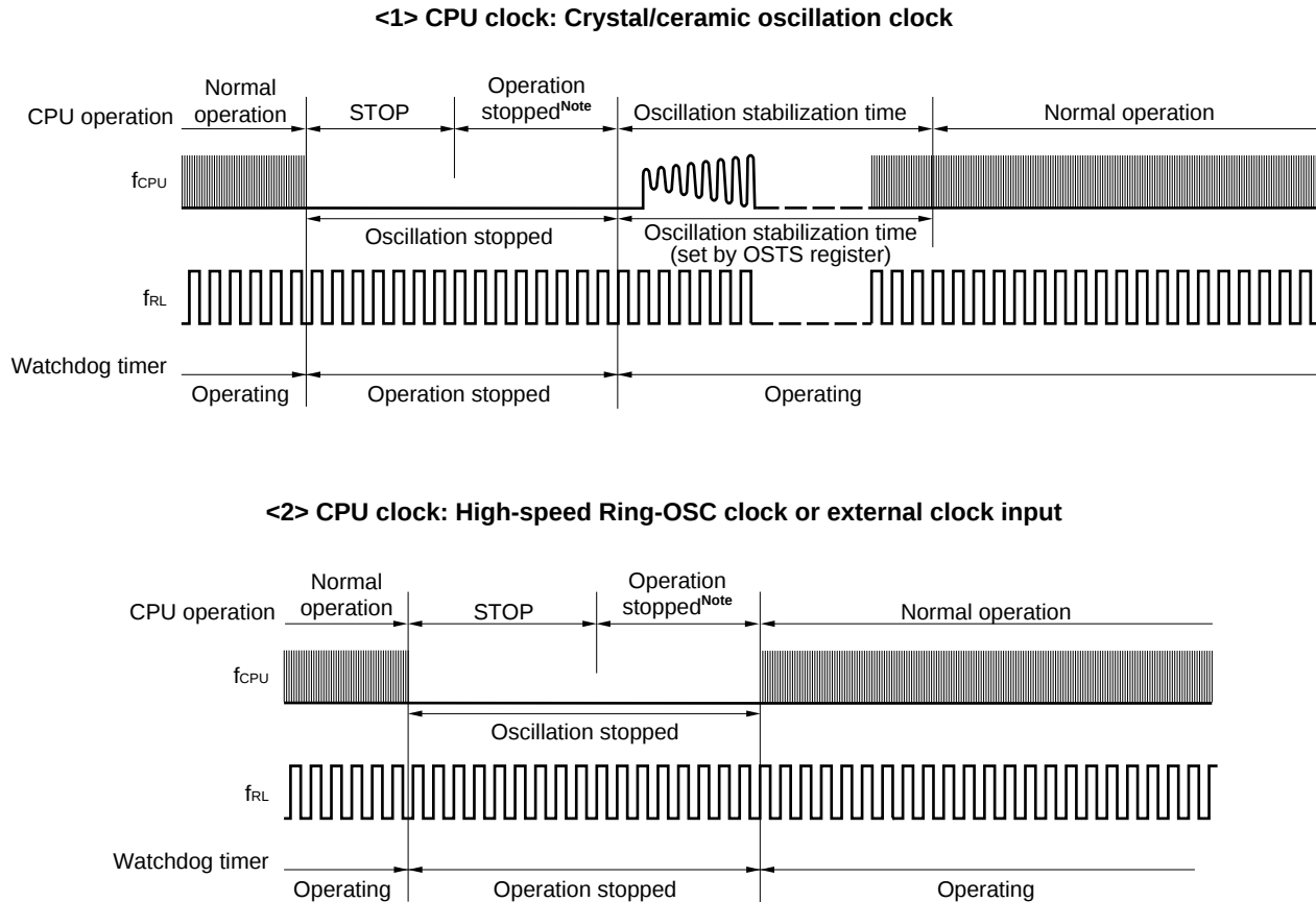
Figure 9-7. Operation in STOP Mode (WDT Operation Clock: Low-Speed Ring-OSC Clock)
