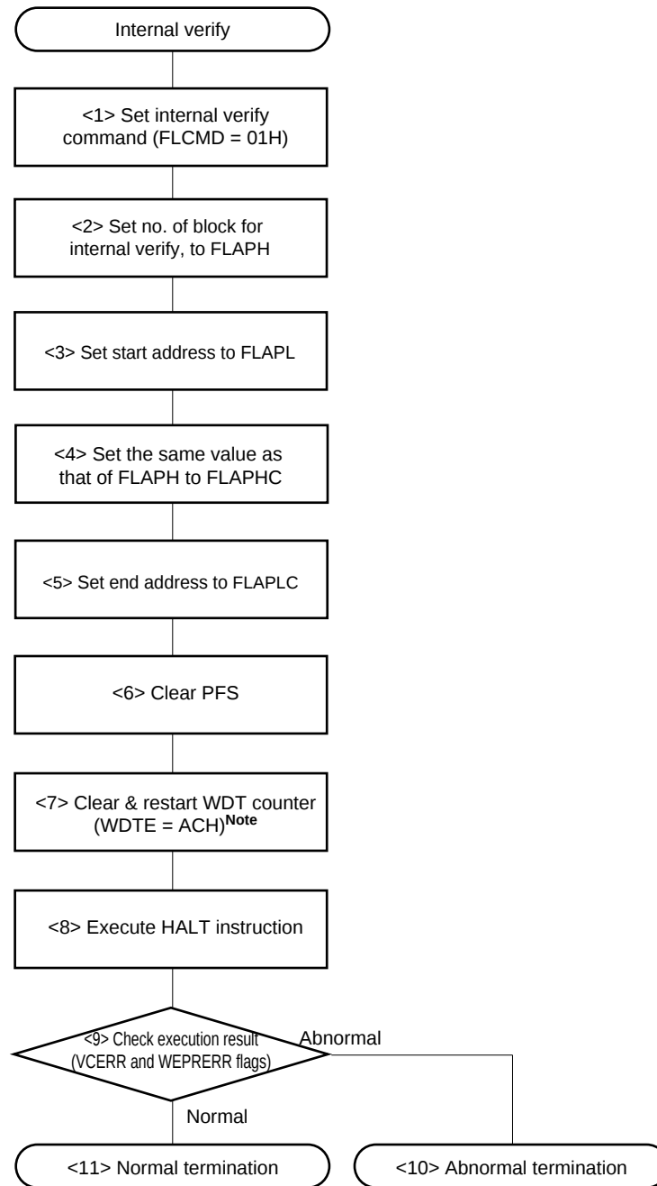
Figure 18-25. Example of Internal Verify Operation in Self Programming Mode
