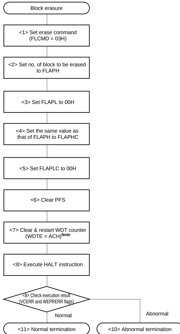
Figure 18-22. Example of Block Erase Operation in Self Programming Mode
