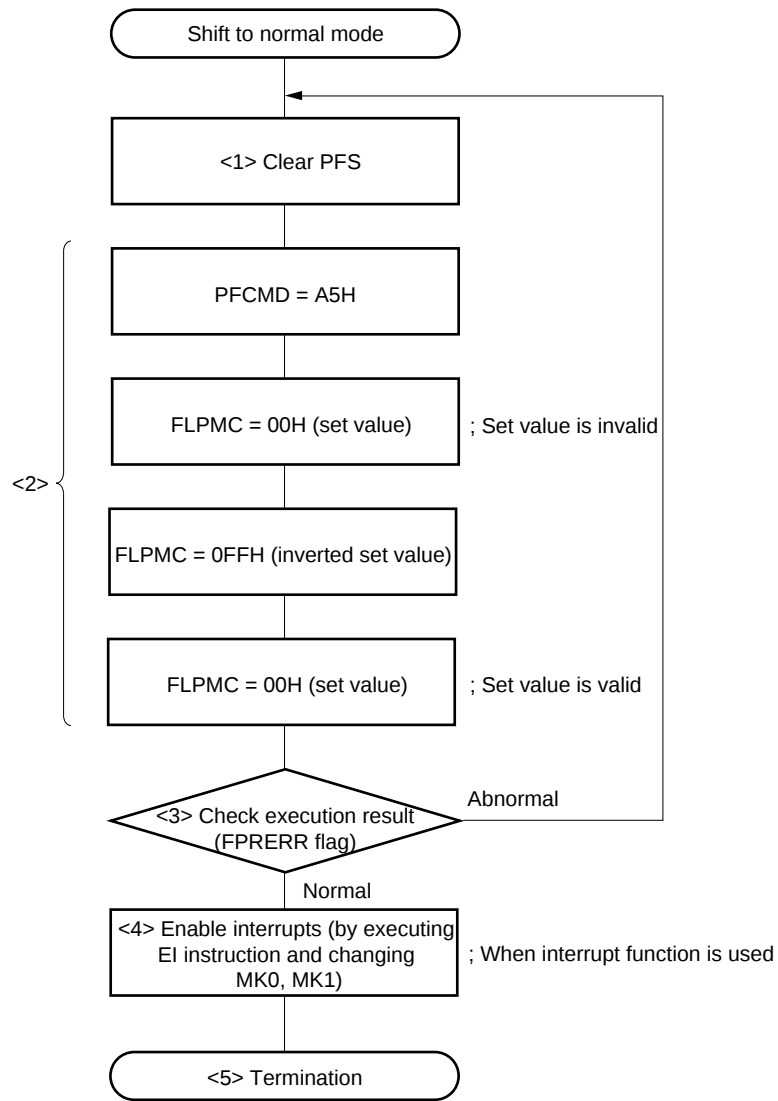
Figure 18-21. Example of Shifting to Normal Mode
