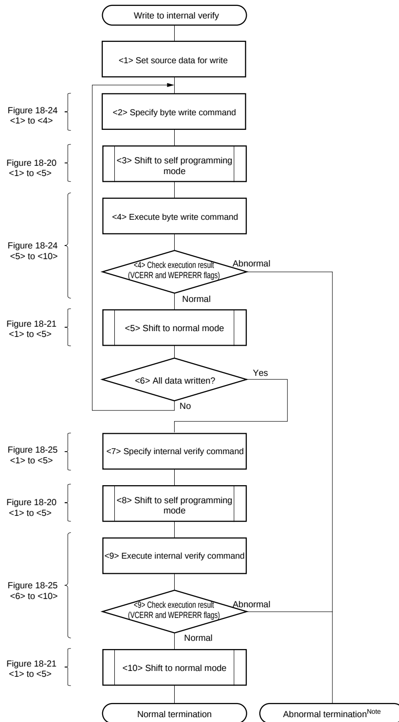
Figure 18-29. Example of Operation When Interrupt-Disabled Time Should Be Minimized (from Write to Internal Verify)
