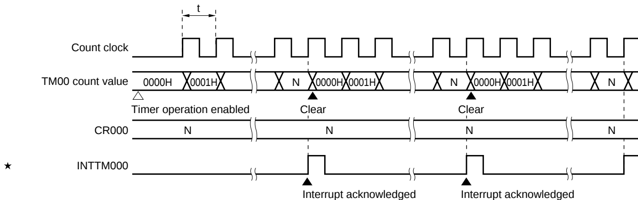
Figure 6-12. Timing of Interval Timer Operation
