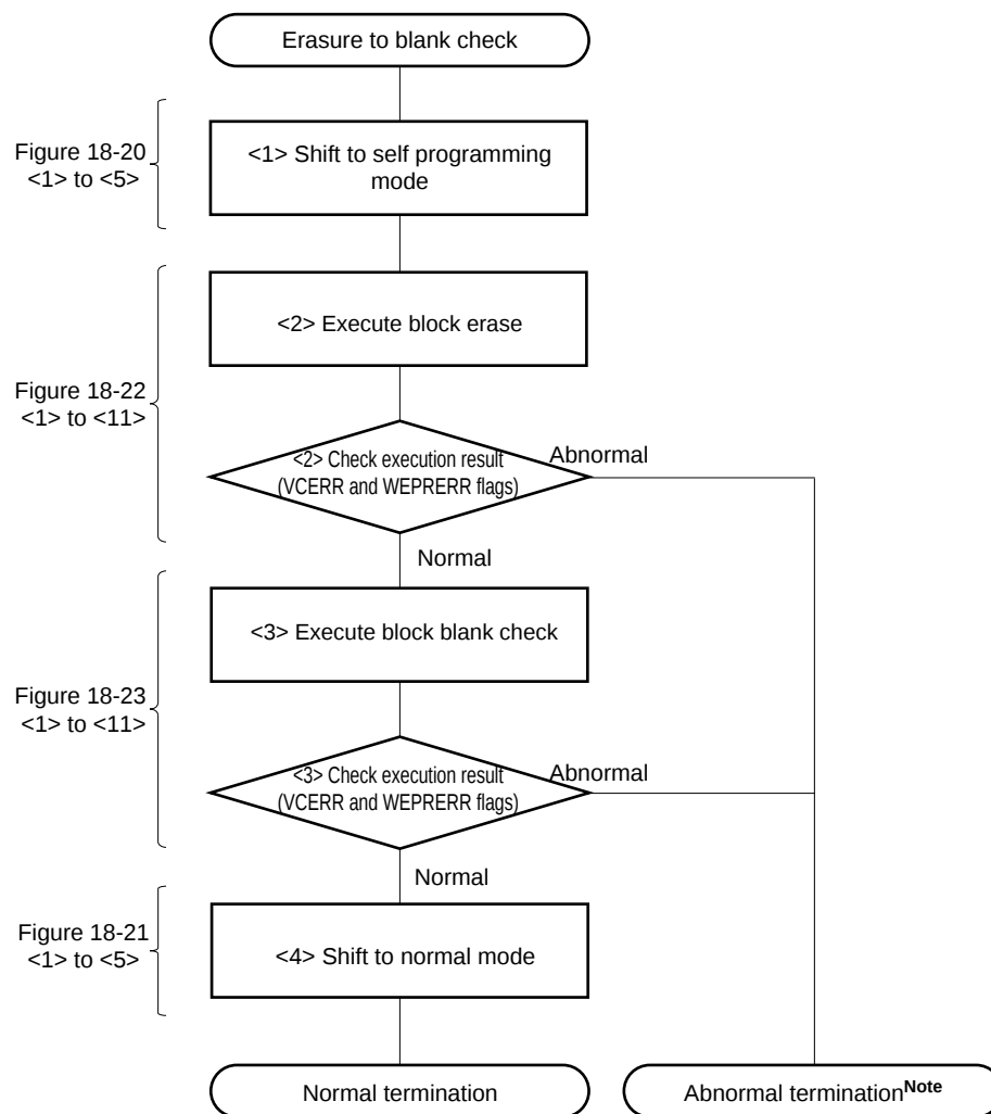
Figure 18-26. Example of Operation When Command Execution Time Should Be Minimized (from Erasure to Blank Check)
