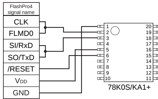
Figure 18-3. Communication with FlashPro4
