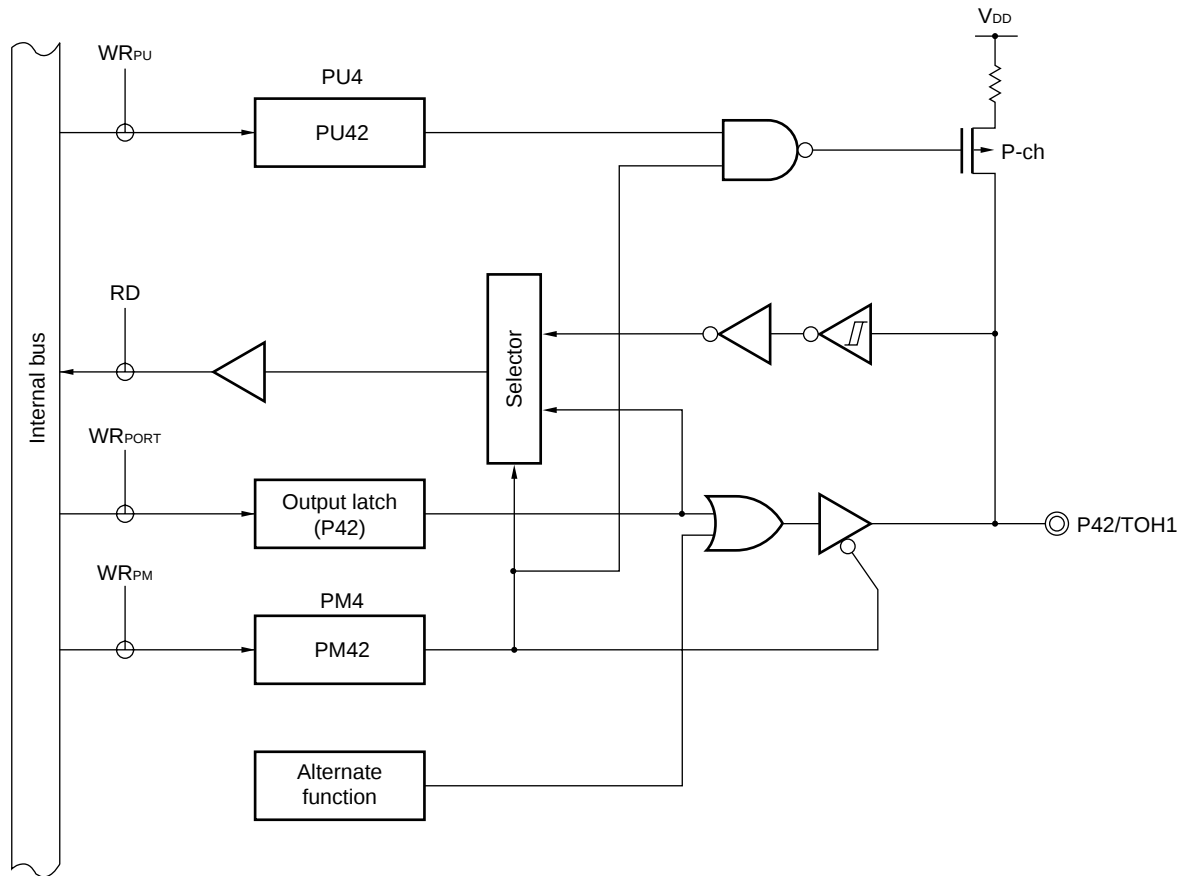
Figure 4-8. Block Diagram of P42
