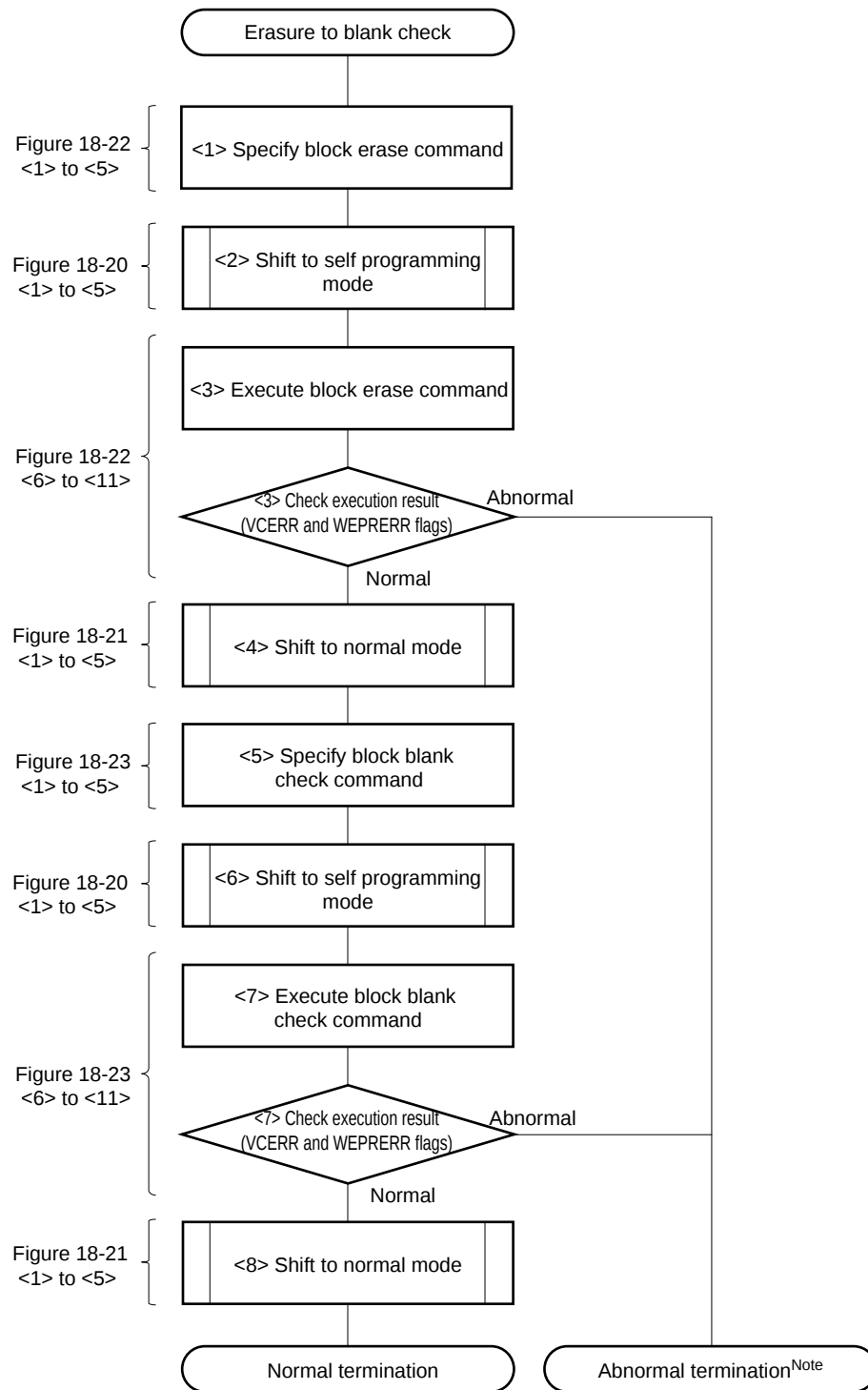
Figure 18-28. Example of Operation When Interrupt-Disabled Time Should Be Minimized (from Erasure to Blank Check)
