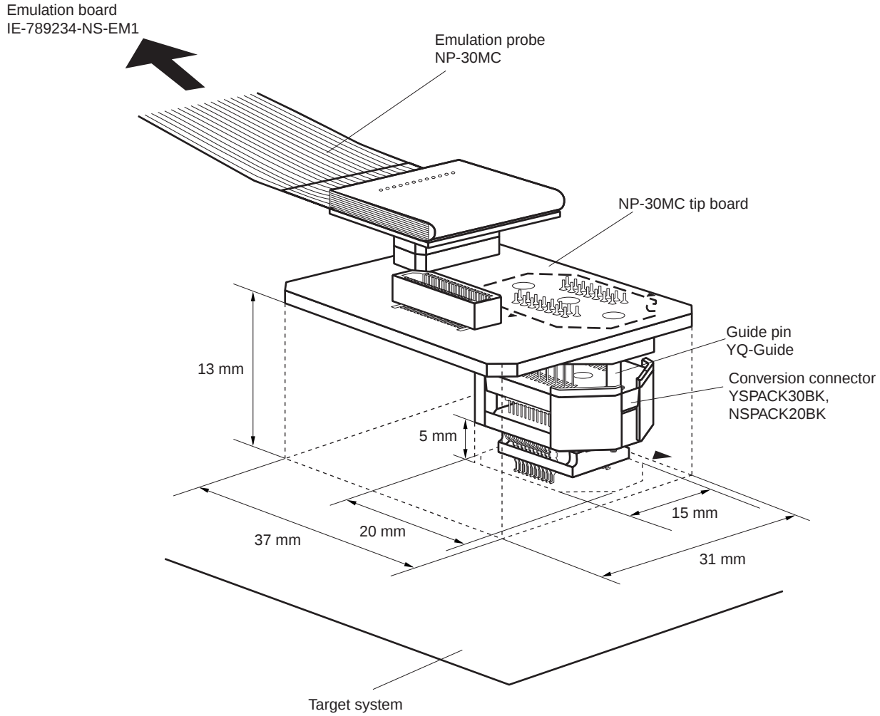
Figure B-2. Condition for Connecting Target System (When Using In-Circuit Emulator IE-78K0S-NS, IE-78K0S-NS-A)
