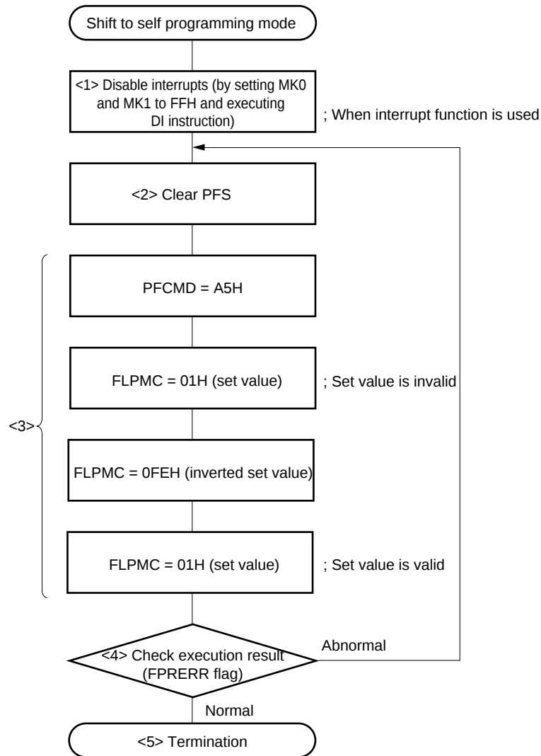
Figure 18-20. Example of Shifting to Self Programming Mode
