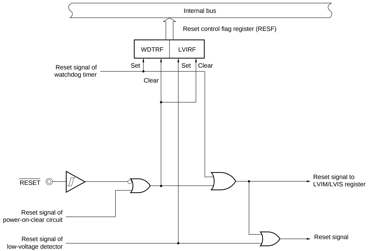
Figure 14-1. Block Diagram of Reset Function
