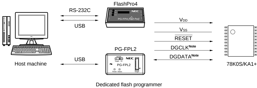
Figure 18-2. Environment for Writing Program to Flash Memory
