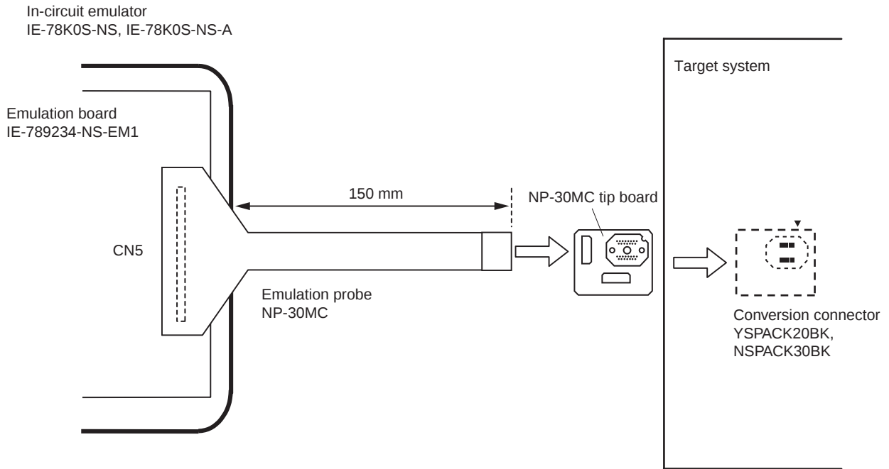
Figure B-1. Distance Between In-Circuit Emulator IE-78K0S-NS/IE-78K0S-NS-A and Conversion Connector NP-30MC
