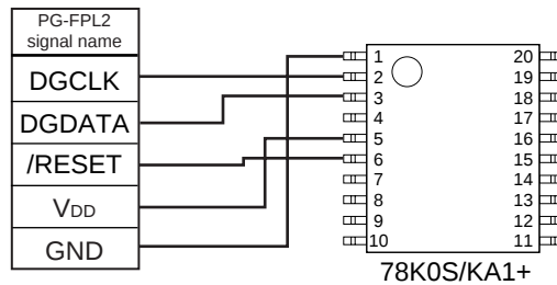
Figure 18-4. Communication with PG-FPL2
