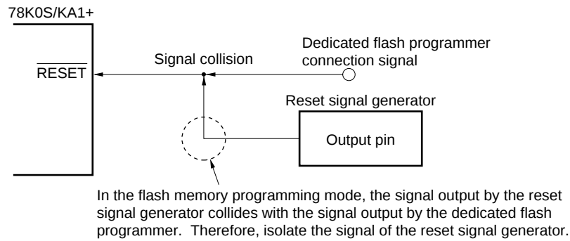
Figure 18-7. Signal Collision (RESET Pin)
