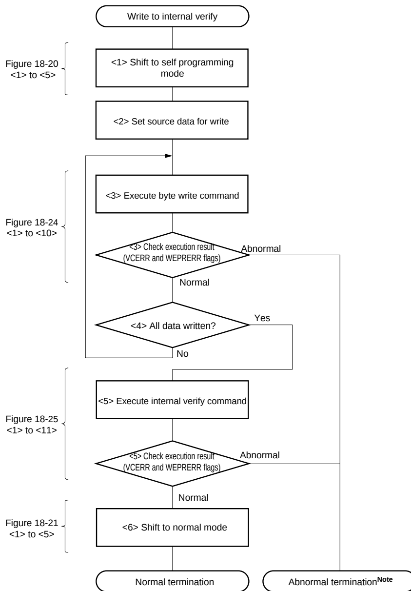
Figure 18-27. Example of Operation When Command Execution Time Should Be Minimized (from Write to Internal Verify)
