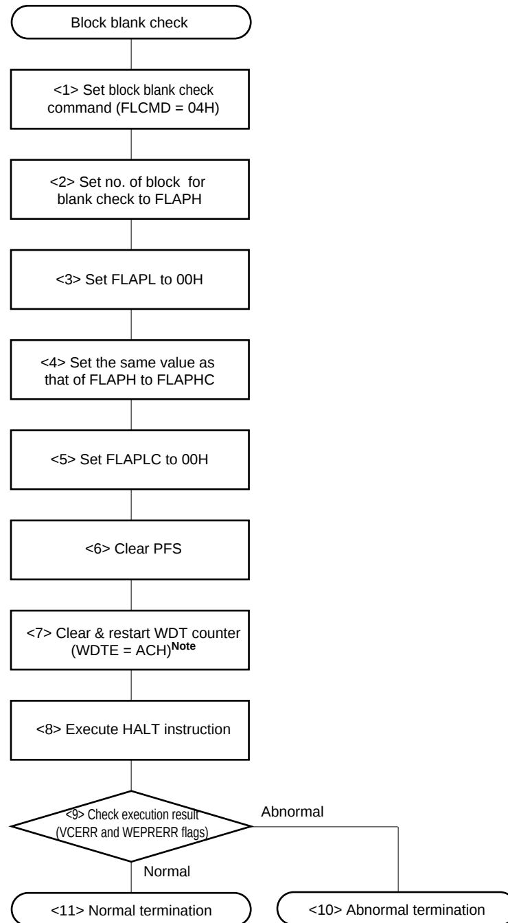
Figure 18-23. Example of Block Blank Check Operation in Self Programming Mode
