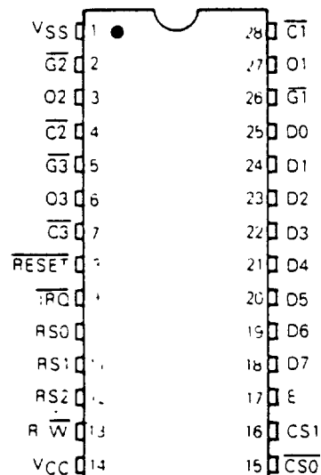
FIGURE 1 — PIN ASSIGNMENT
