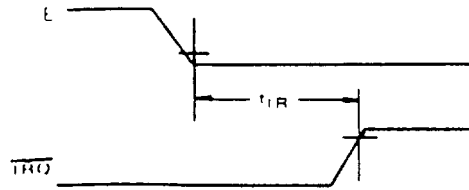
FIGURE 8 – \overline{IRQ} RELEASE TIME
