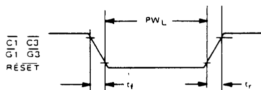
FIGURE 4 — INPUT PULSE WIDTH LOW
