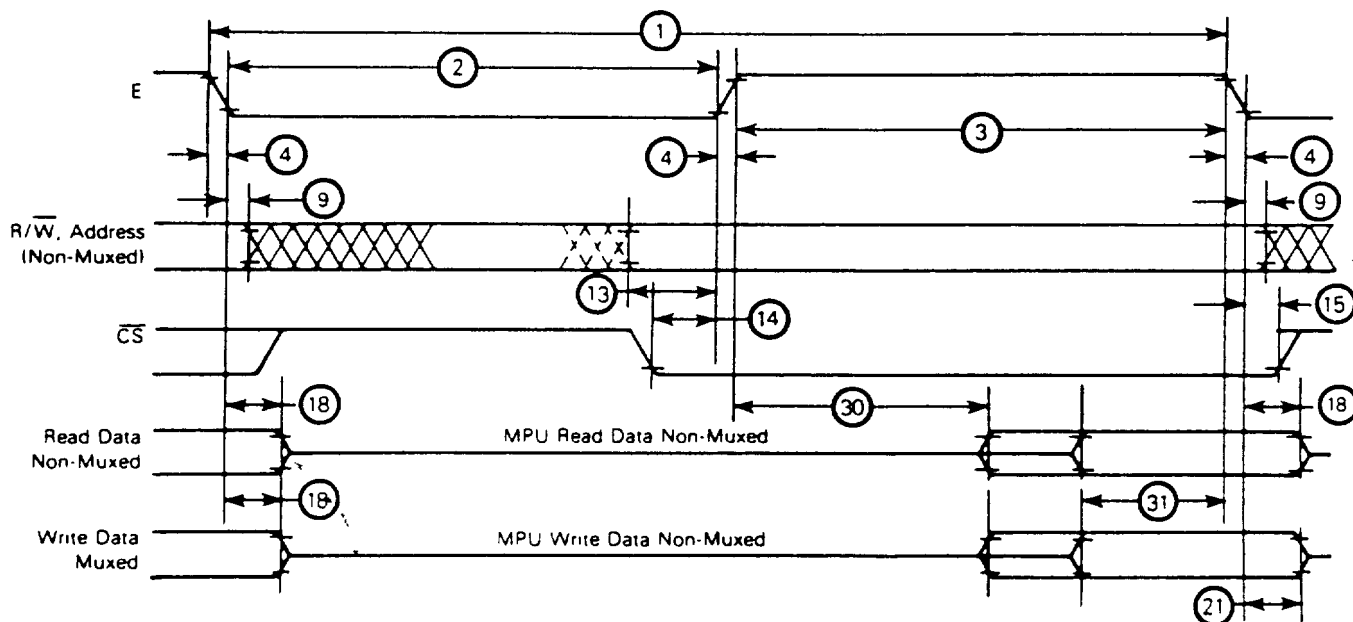
FIGURE 3 — BUS TIMING
