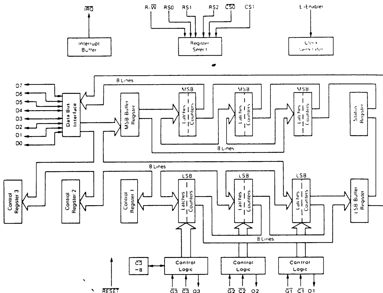
FIGURE 2 — BLOCK DIAGRAM
