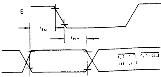
FIGURE 6 – INPUT SETUP AND HOLD TIMES
