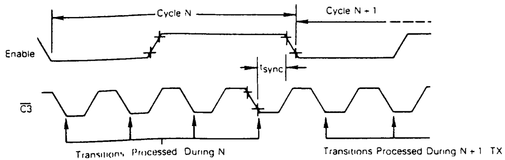
FIGURE 9 – \overline{C3} INPUT SYNCHRONIZATION TIME (– 8 PRESCALER MODE ONLY)
