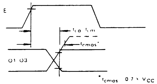
FIGURE 7 – OUTPUT DELAY
