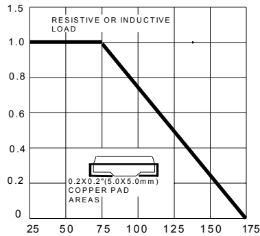
FIG.1 – FORWARD CURRENT DERATING CURV
