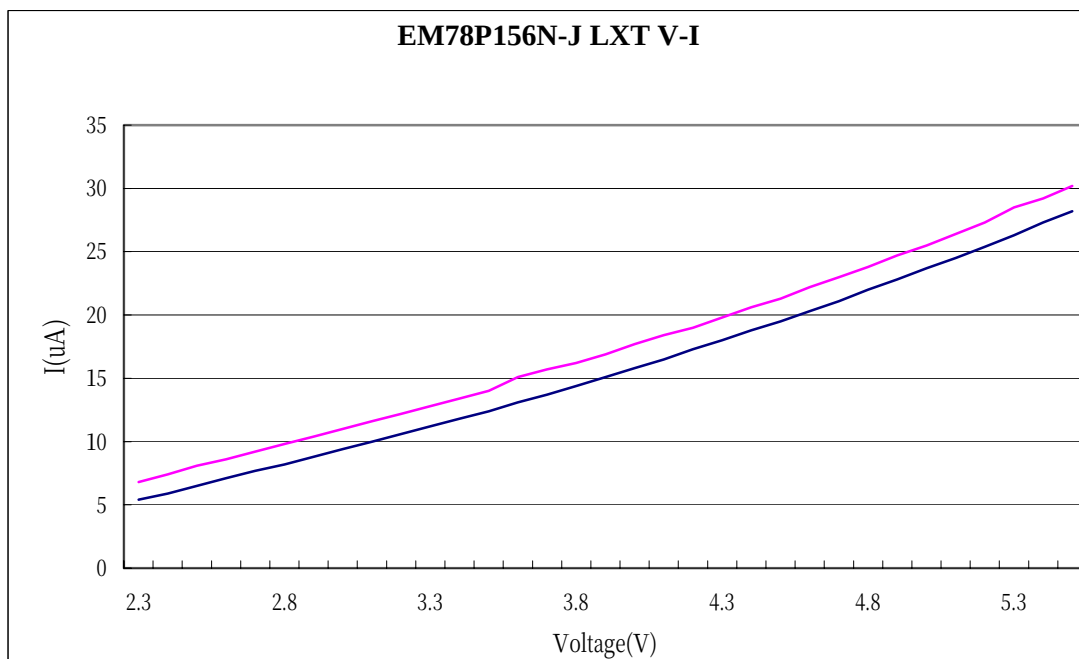
Fig. 35 Operating current range (based on low Freq. @ =25°C) vs. Voltage
