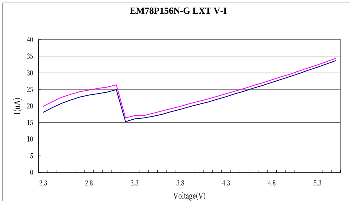
Fig. 37 Operating current range (based on high Freq. @ =25°C) vs. Voltage
