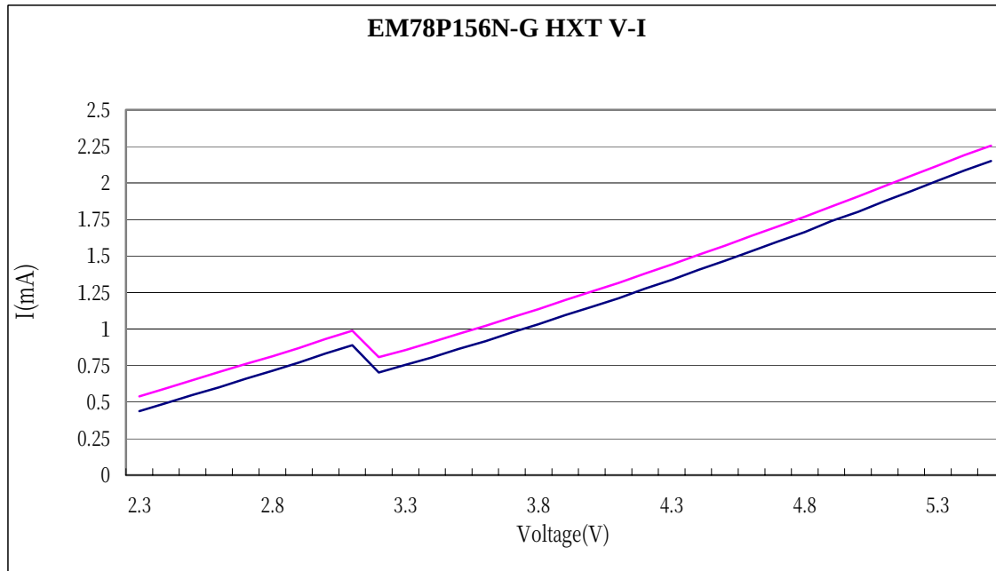
Fig. 36 Operating current range (based on high Freq. @ =25°C) vs. Voltage
