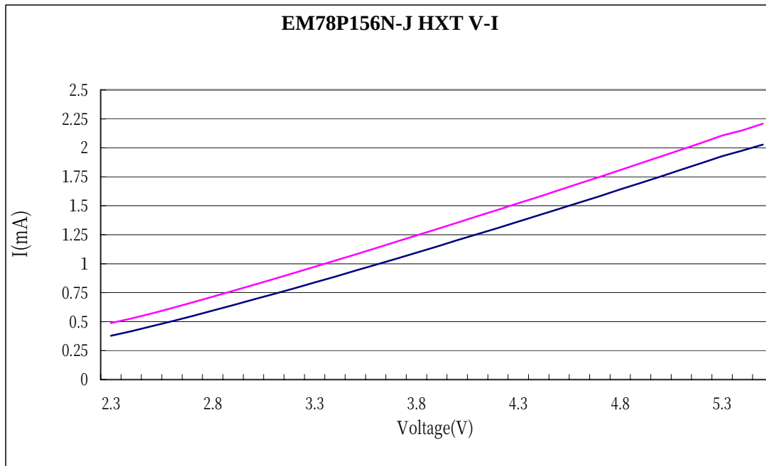
Fig. 34 Operating current range (based on high Freq. @ =25°C) vs. Voltage
