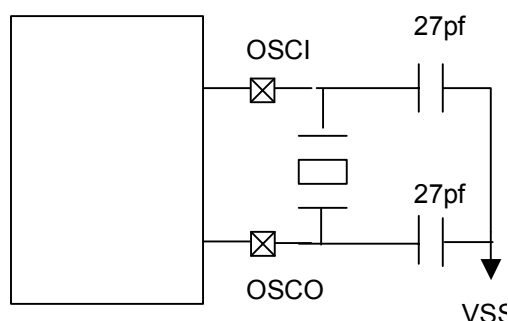
Fig. 15 Crystal OSC Block Diagram
