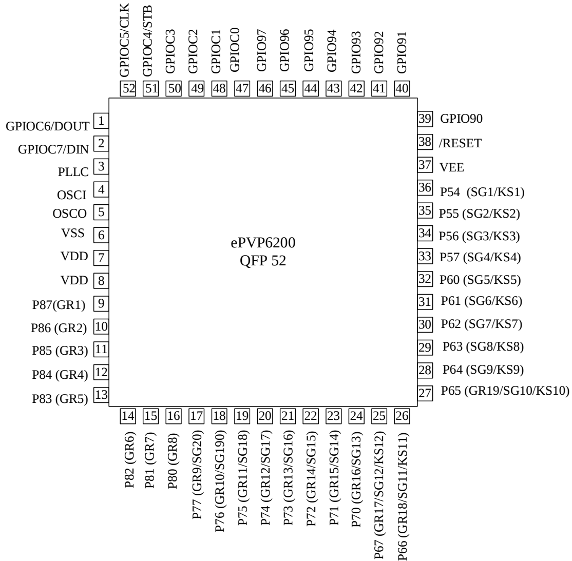
Fig. 1 Pin Assignment
