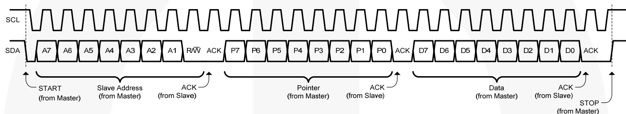
Figure 7. I²C Write
