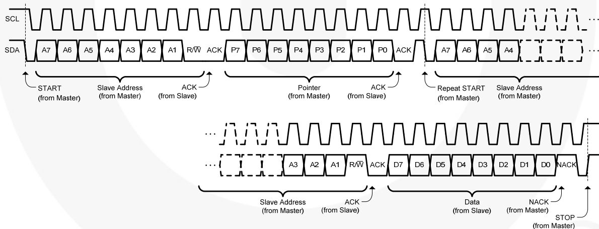
Figure 8. I²C Write Followed by Read
