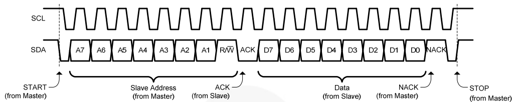
Figure 5. I²C Read
