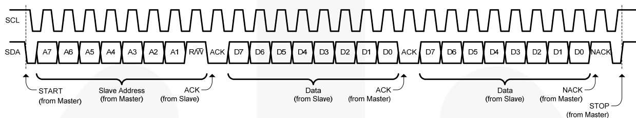
Figure 6. I²C Multiple Byte Read
