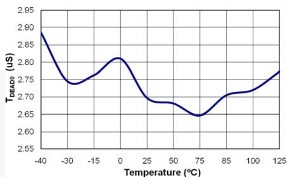
Figure 7. PWM Dead Time 2μs (t DEAD0 ) vs. Temperature
