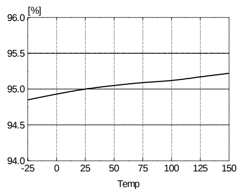
Figure 6. Maximum Duty vs. Temp.
