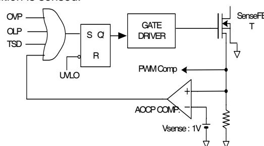
Figure 25. AOCP block
