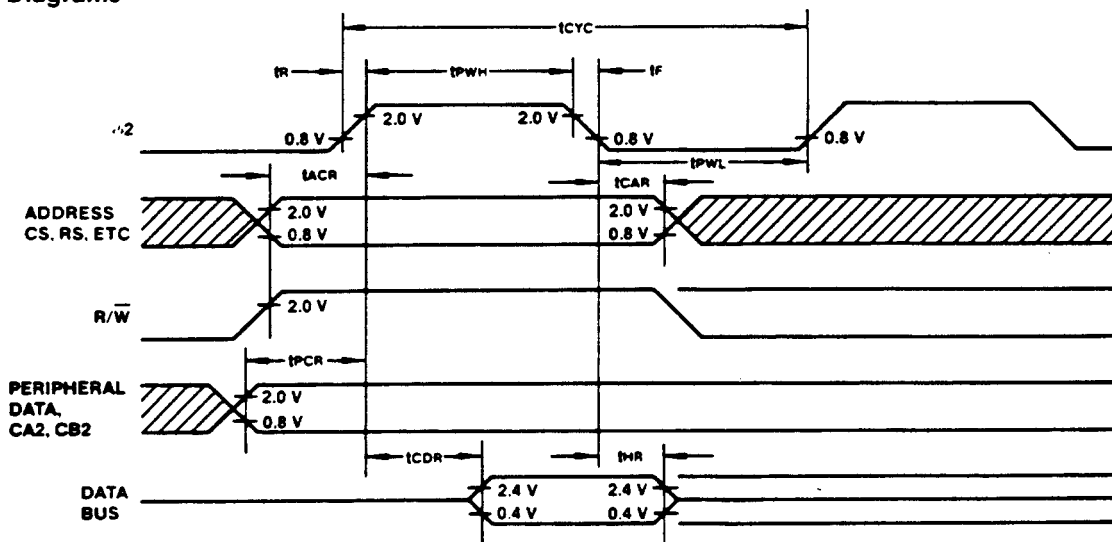
Figure 1. Read Timing
