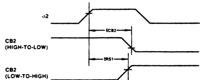
Figure 6. CB2 Timing
