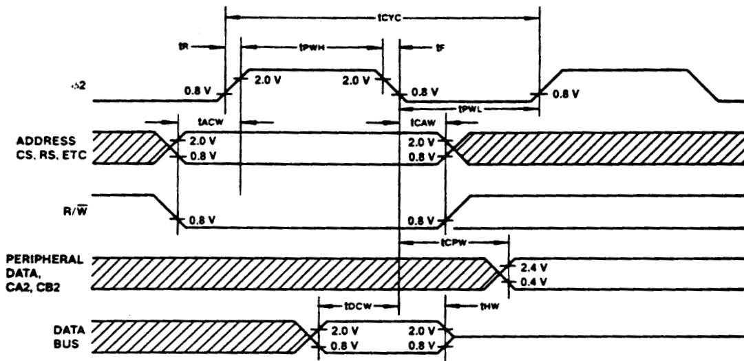
Figure 2. Write Timing
