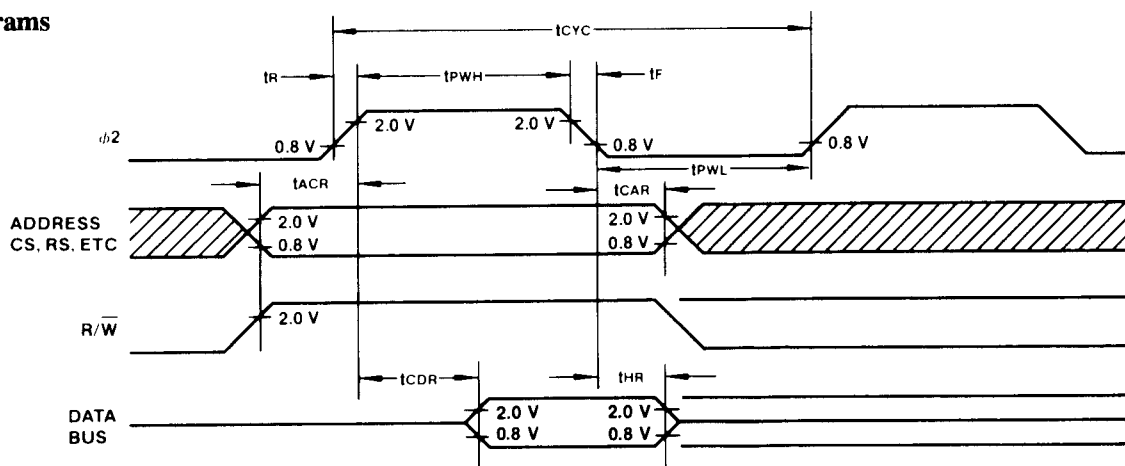
Figure 1. Read Timing
