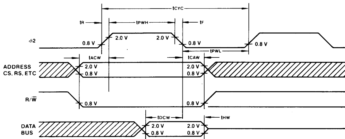
Figure 2. Write Timing
