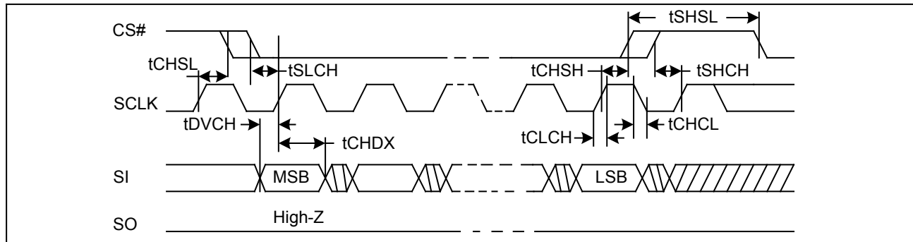
Figure 32. Output Timing
