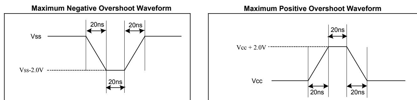
Figure 30. Input Test Waveform and Measurement Level
