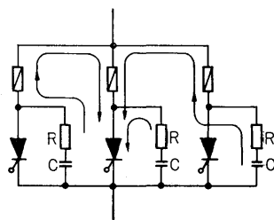
Fig. 17 Connection of R-C filter
