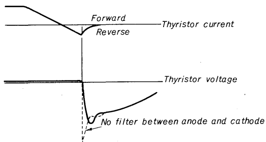
Fig. 18 Transient waveforms of thyristor current and voltage at turn-off
