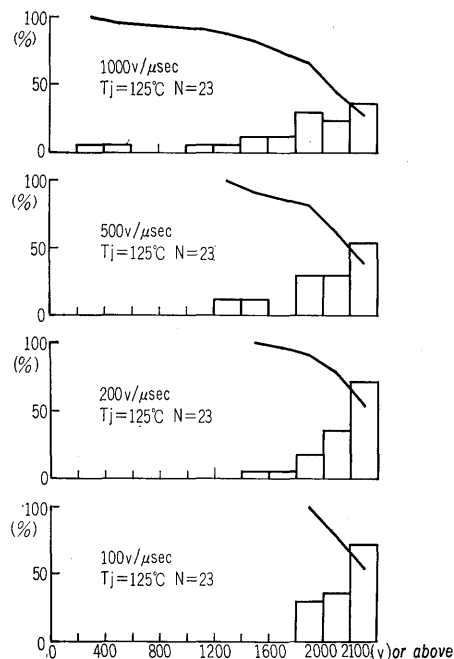
Fig. 4 Forward blocking voltage of KGP02 for various dv/dt
