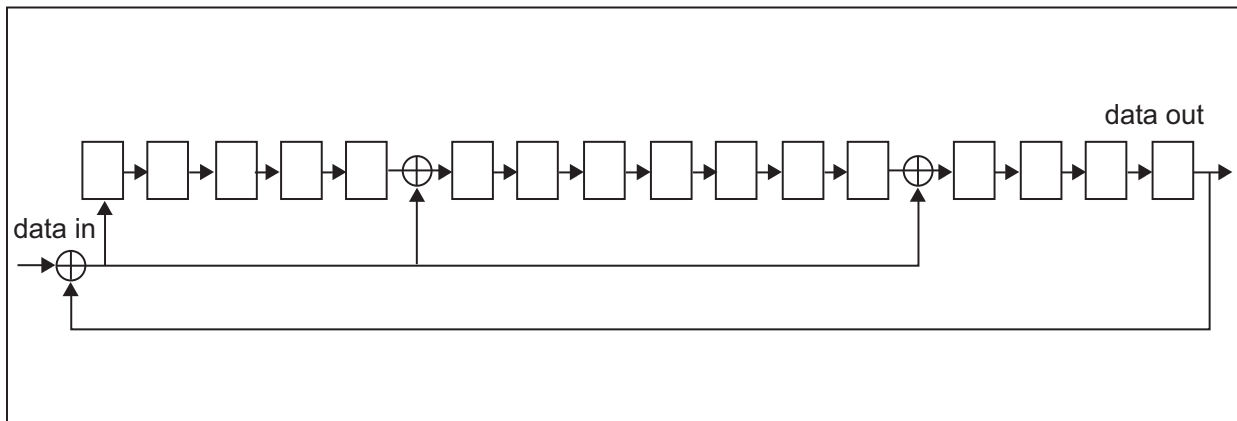
Figure 4-8 : CRC16 Generator/Checker
