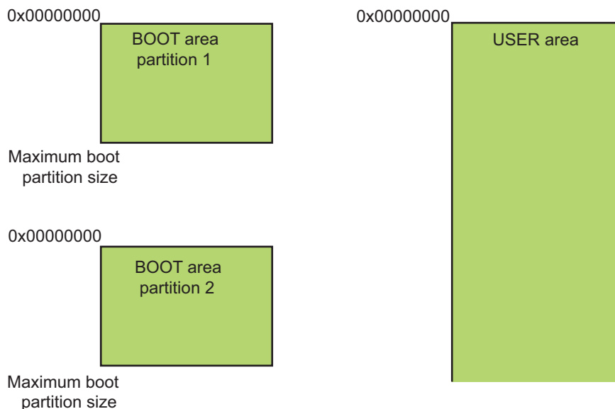
Figure 4-1: Memory partition
