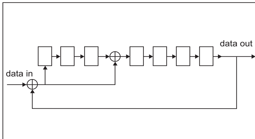
Figure 4-7 : CRC7 Generator/Checker
