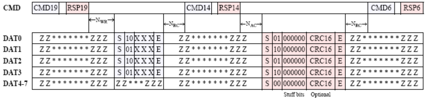
Figure 4-25 : 4 bit System Bus Testing Procedure
